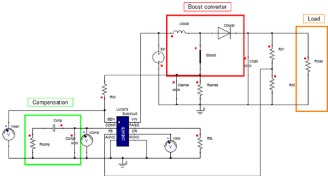
Figure 2. Example Circuit
