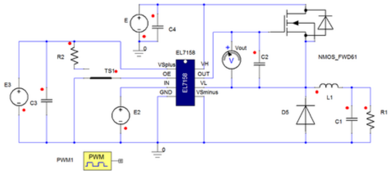
Figure 2. Example Circuit
