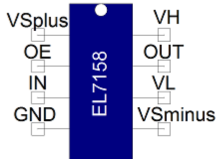
Figure 1. Component symbol
