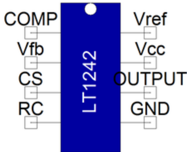
Figure 1. Component symbol
