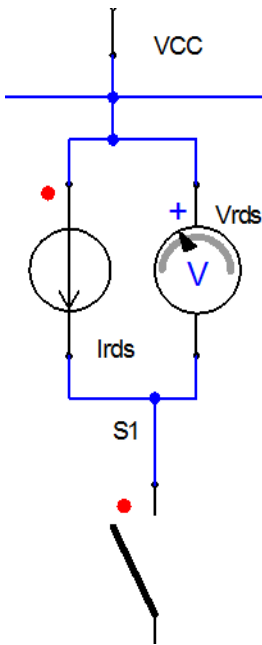
Figure 2. Partial View of the Block Diagram
