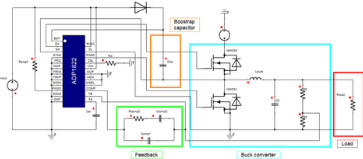
Figure 2. Example Circuit
