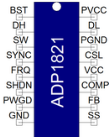
Figure 1. Component symbol
