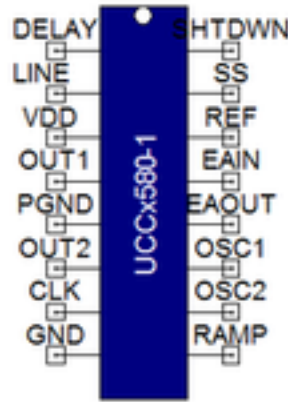
Figure 1. Component symbol
