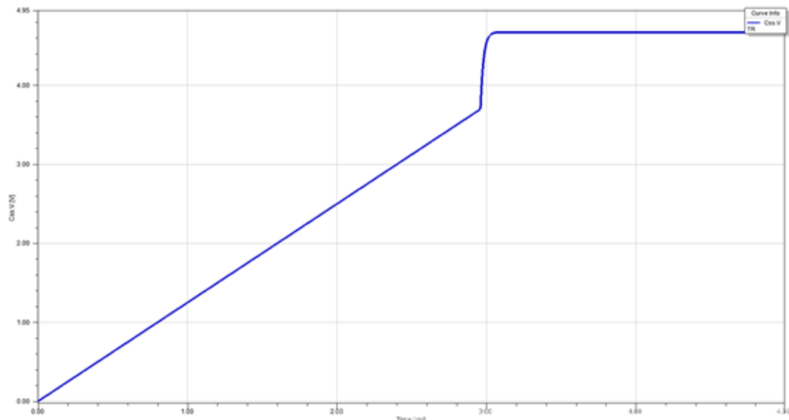
Figure 3. Soft Start Pin Voltage
