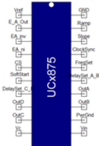
Figure 1. Component symbol
