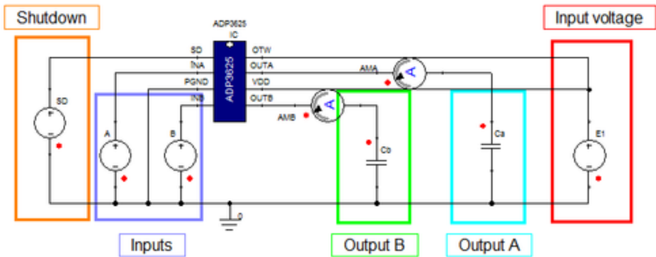
Figure 2. Example Circuit
