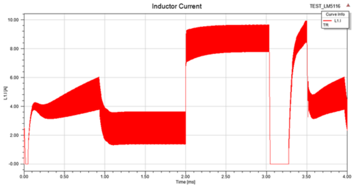
Figure 4: Inductor Current
