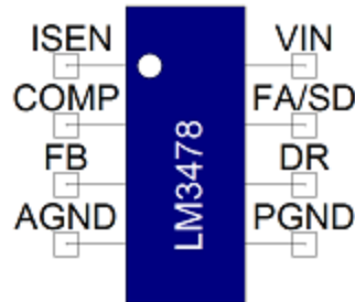
Figure 1. Component symbol
