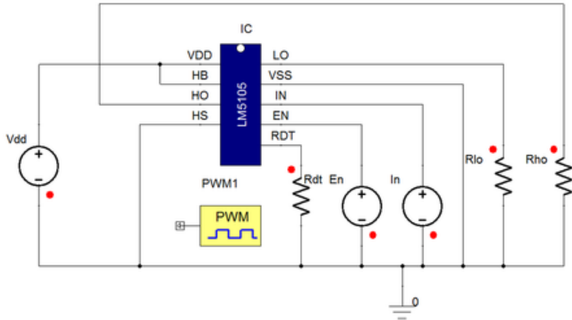
Figure 2. Example Circuit
