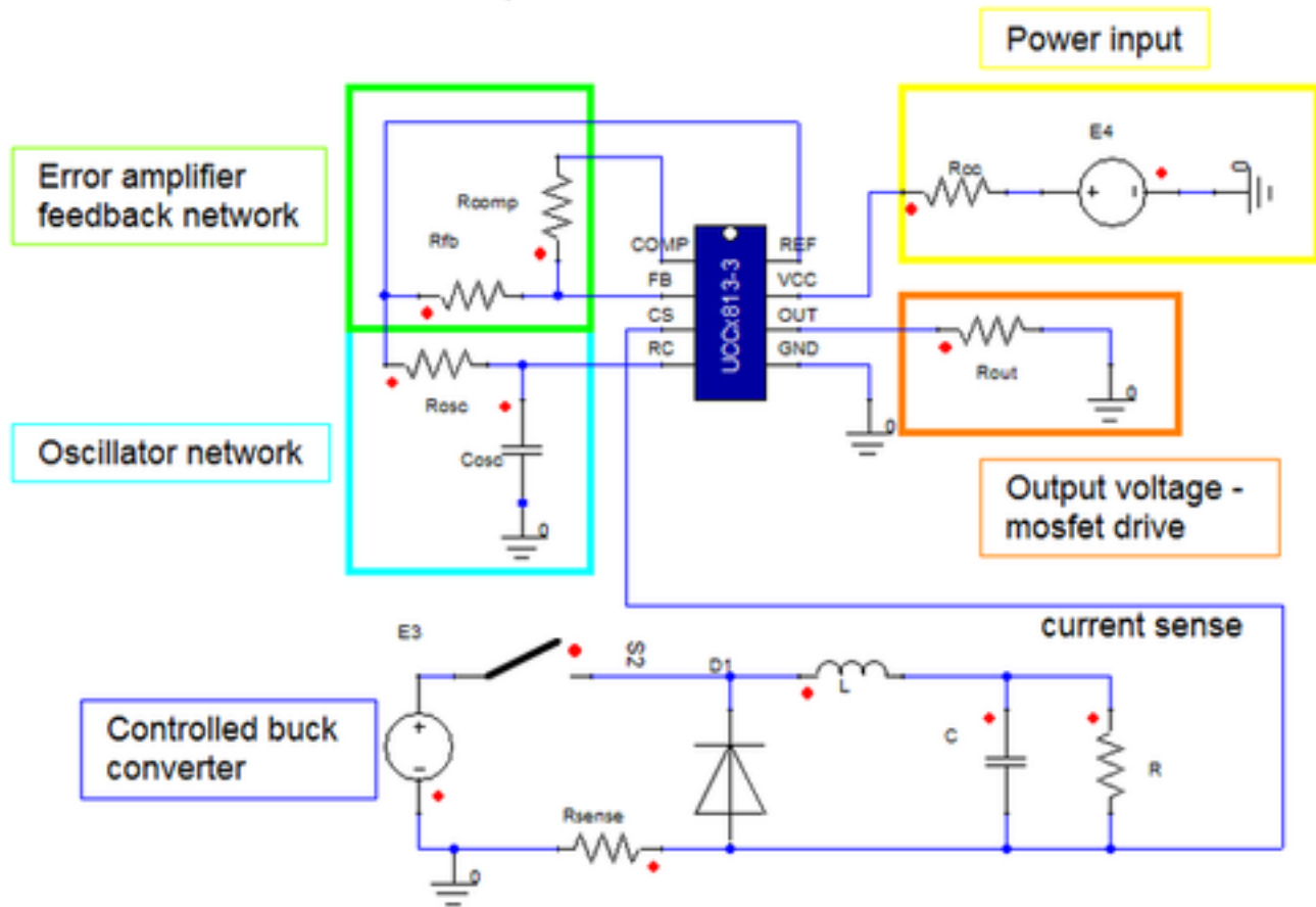
Figure 2. Example Circuit
