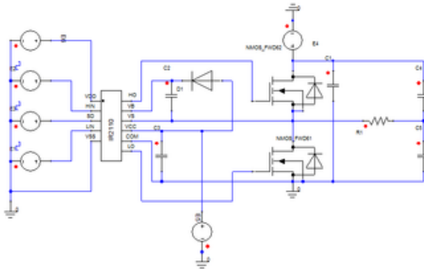
Figure 2. Example Circuit
