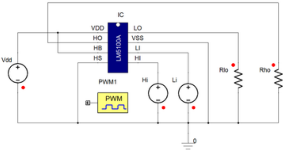
Figure 2. Example Circuit
