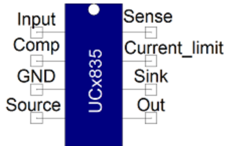
Figure 1. Component symbol
