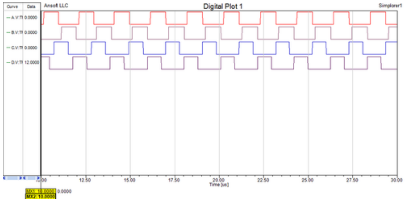
Figure 4. Simulation results(a)
