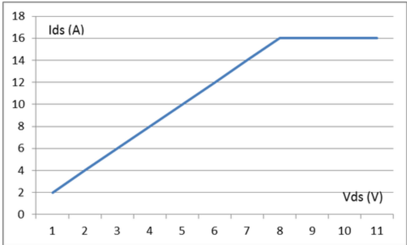
Figure 3. Conduction Resistance Curve
