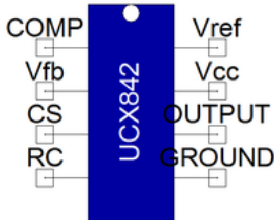
Figure 1. Component symbol
