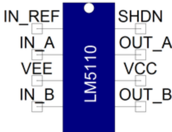
Figure 1. Component symbol
