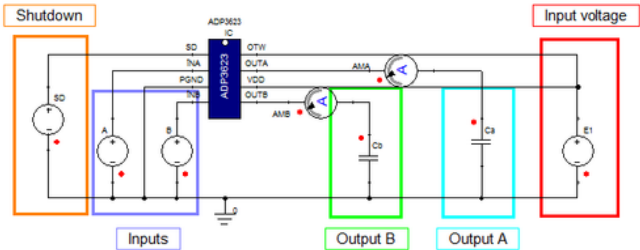
Figure 2. Example Circuit
