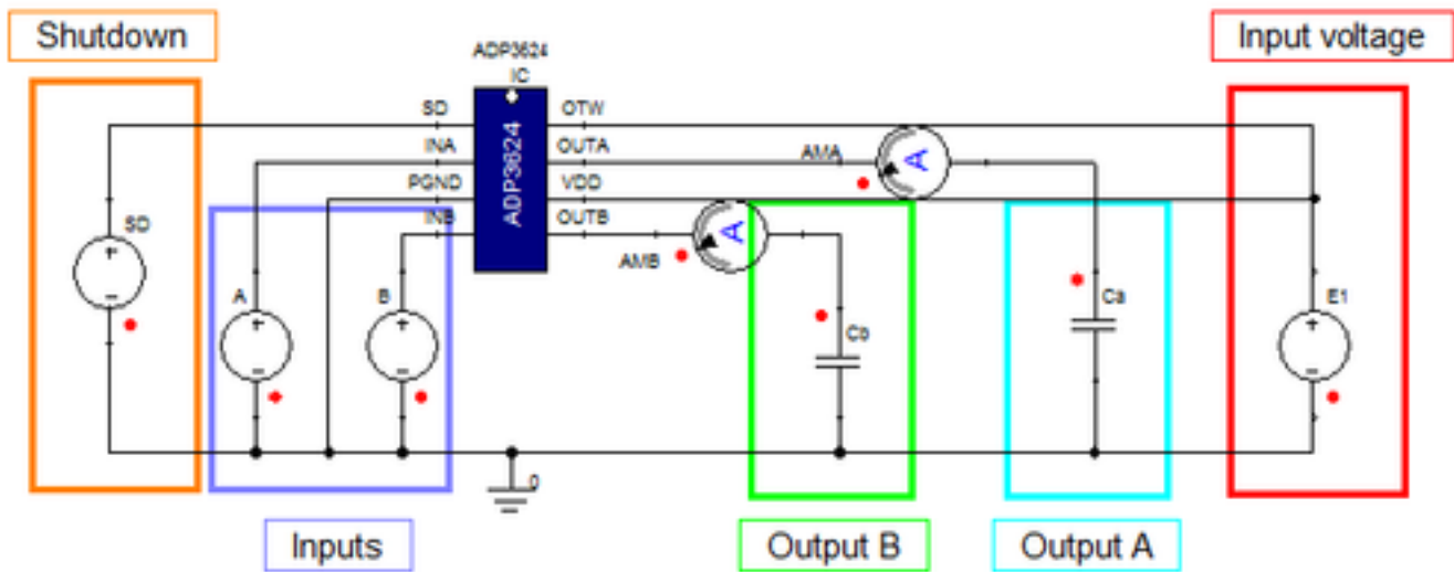
Figure 2. Example Circuit
