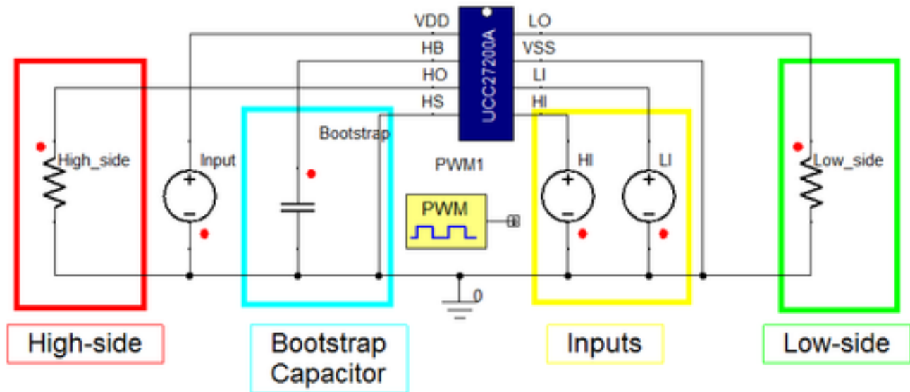
Figure 2. Example Circuit
