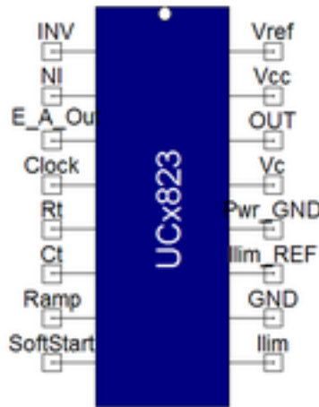
Figure 1. Component symbol
