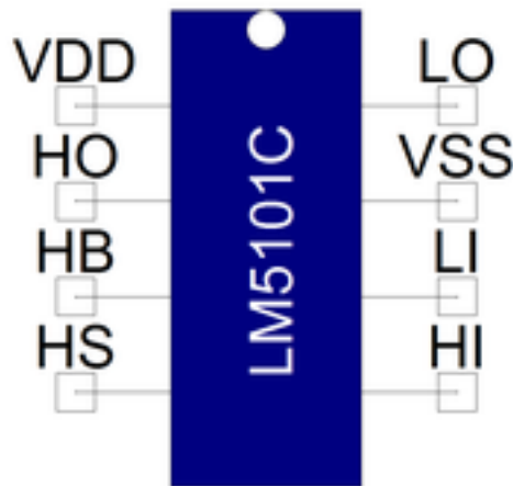
Figure 1. Component symbol
