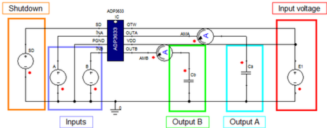
Figure 2. Example Circuit
