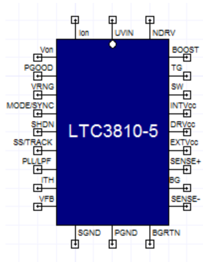
Figure 1. Component symbol
