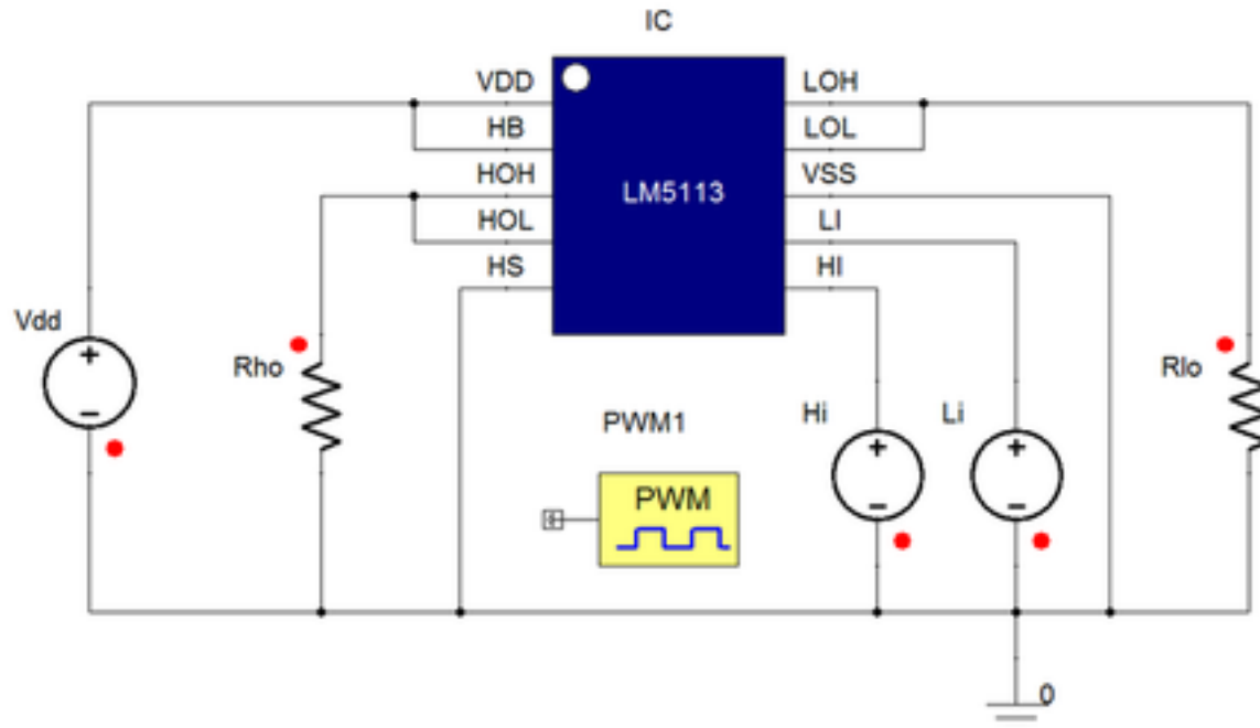
Figure 2. Example Circuit
