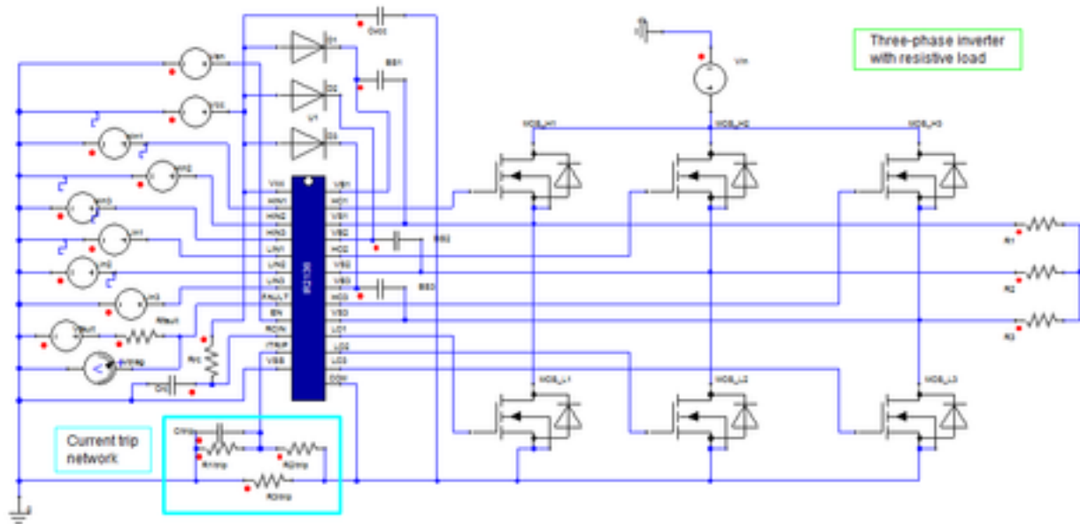
Figure 2. Example Circuit
