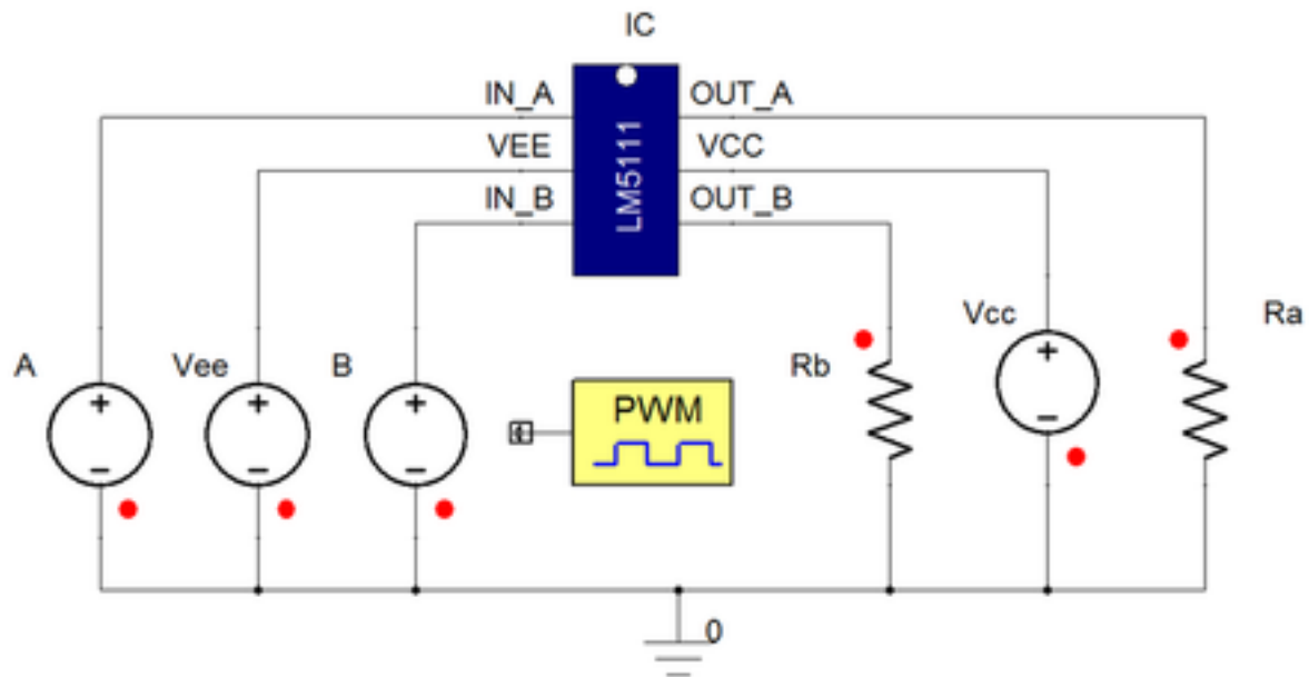
Figure 2. Example Circuit
