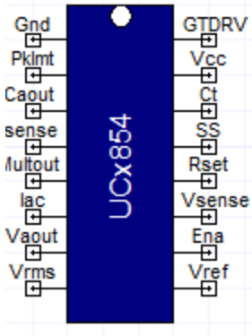
Figure 1. Component symbol
