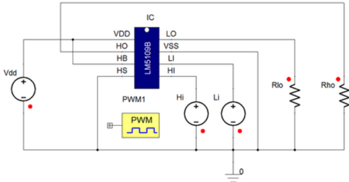
Figure 2. Example Circuit
