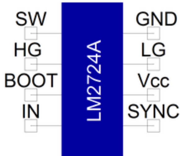
Figure 1. Component symbol
