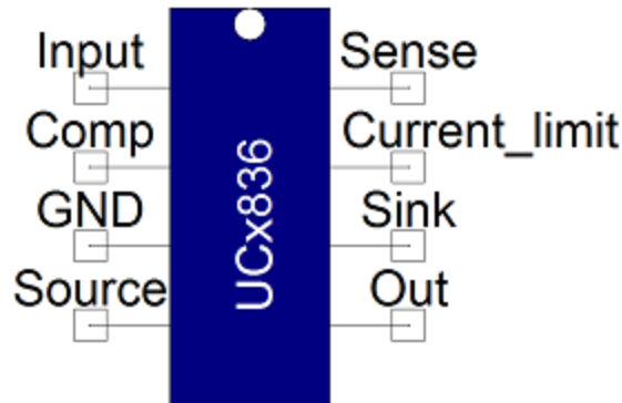
Figure 1. Component symbol
