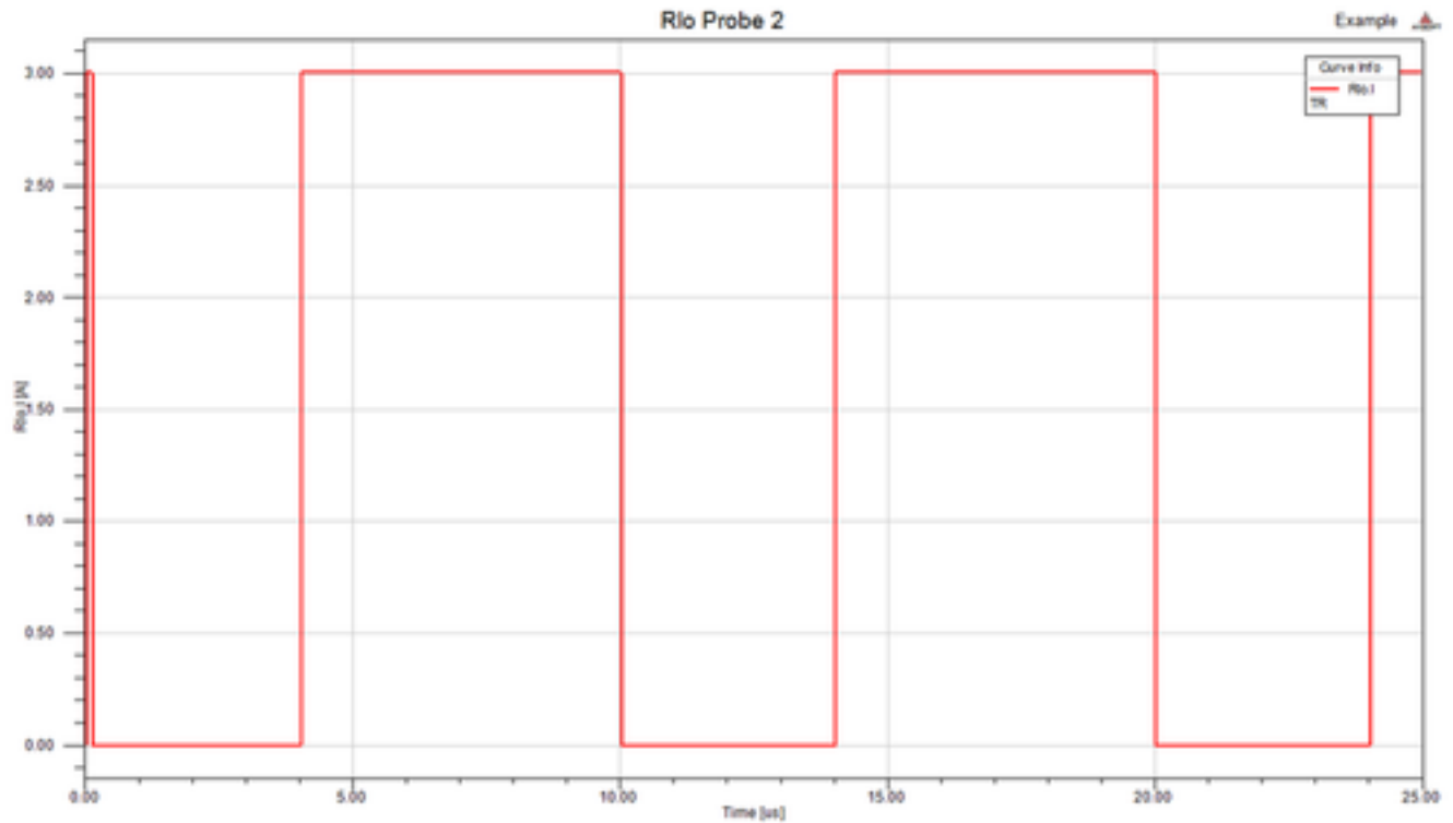
Figure 3. Simulation results
