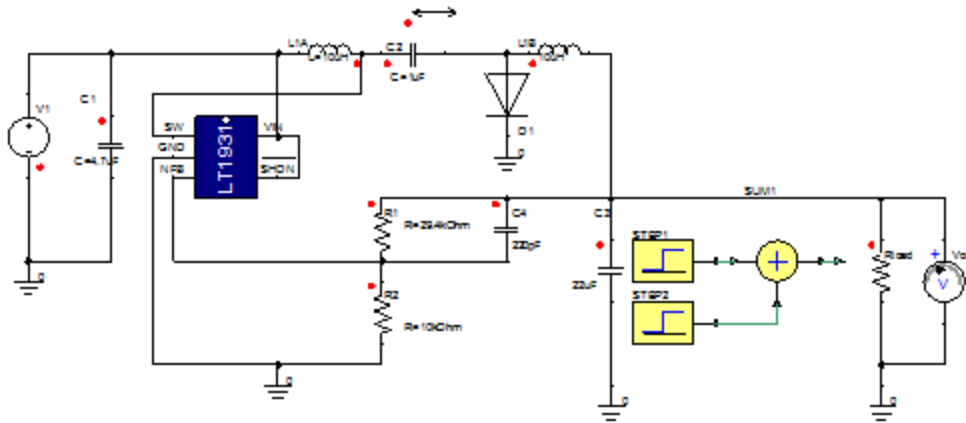
Figure 2. Example of Connection
