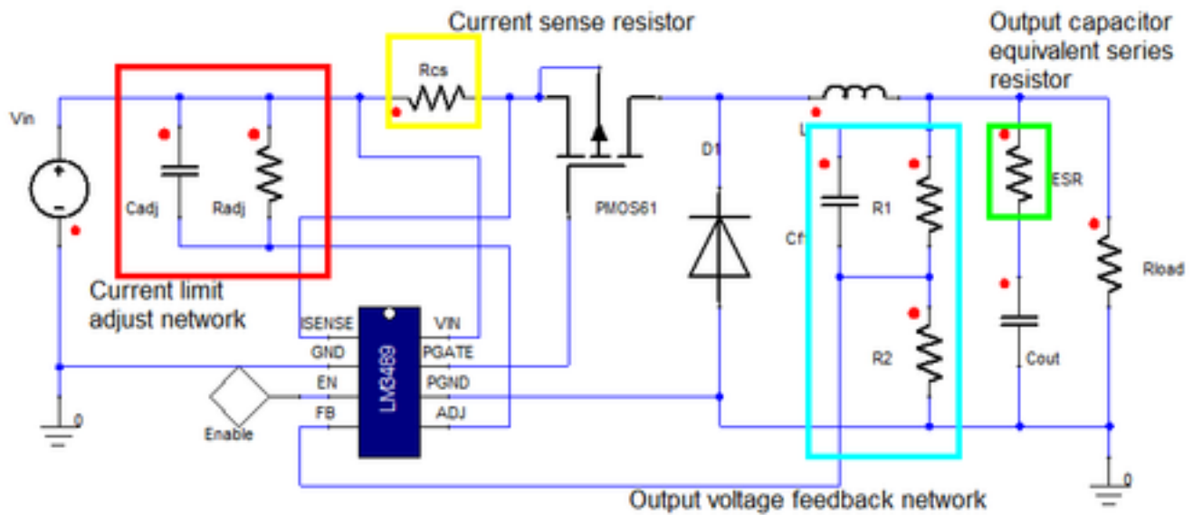
Figure 2. Example Circuit
