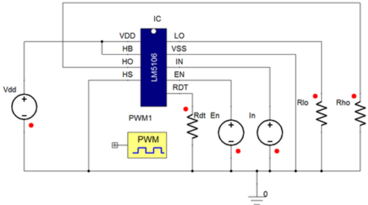
Figure 2. Example Circuit
