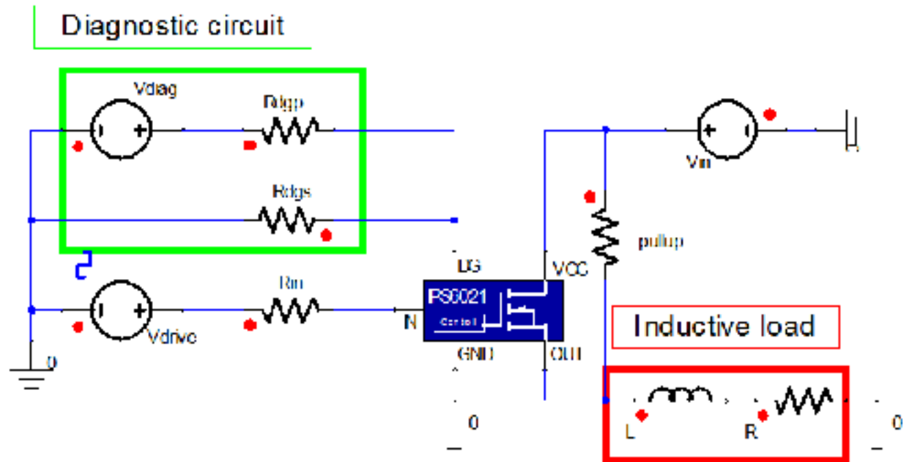
Figure 4. Example Circuit
