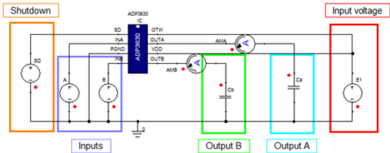
Figure 2. Example Circuit
