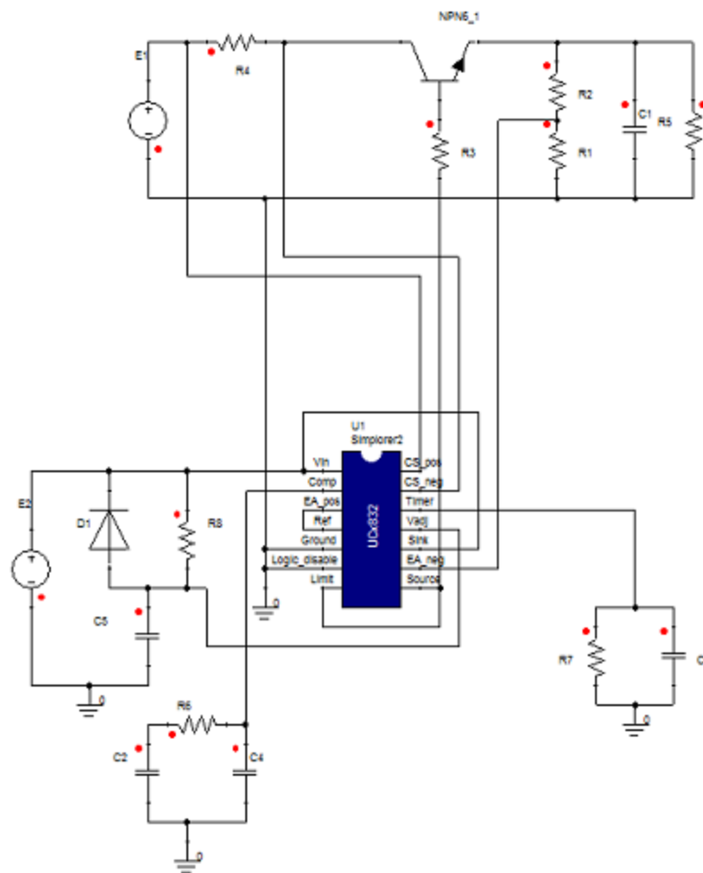
Figure 2. Example Circuit
