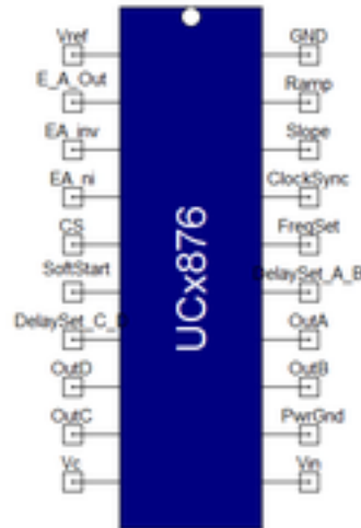
Figure 1. Component symbol
