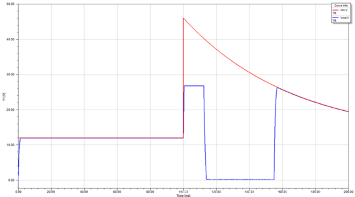
Figure 4. Input and Output Voltage
