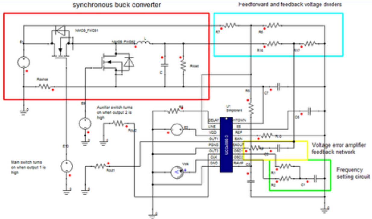
Figure 2. Example Circuit
