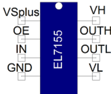
Figure 1. Component symbol
