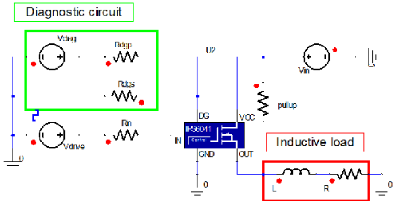
Figure 4. Example Circuit
