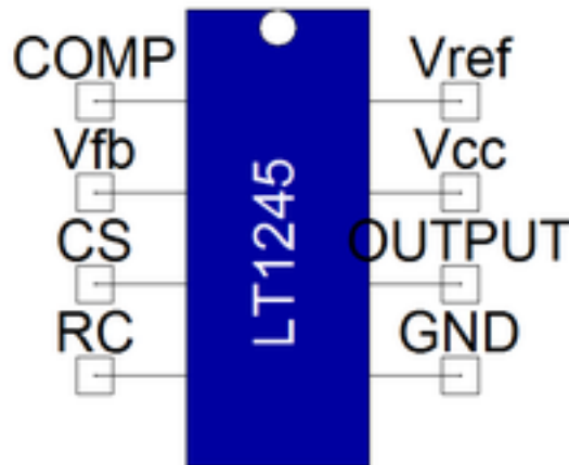
Figure 1. Component symbol
