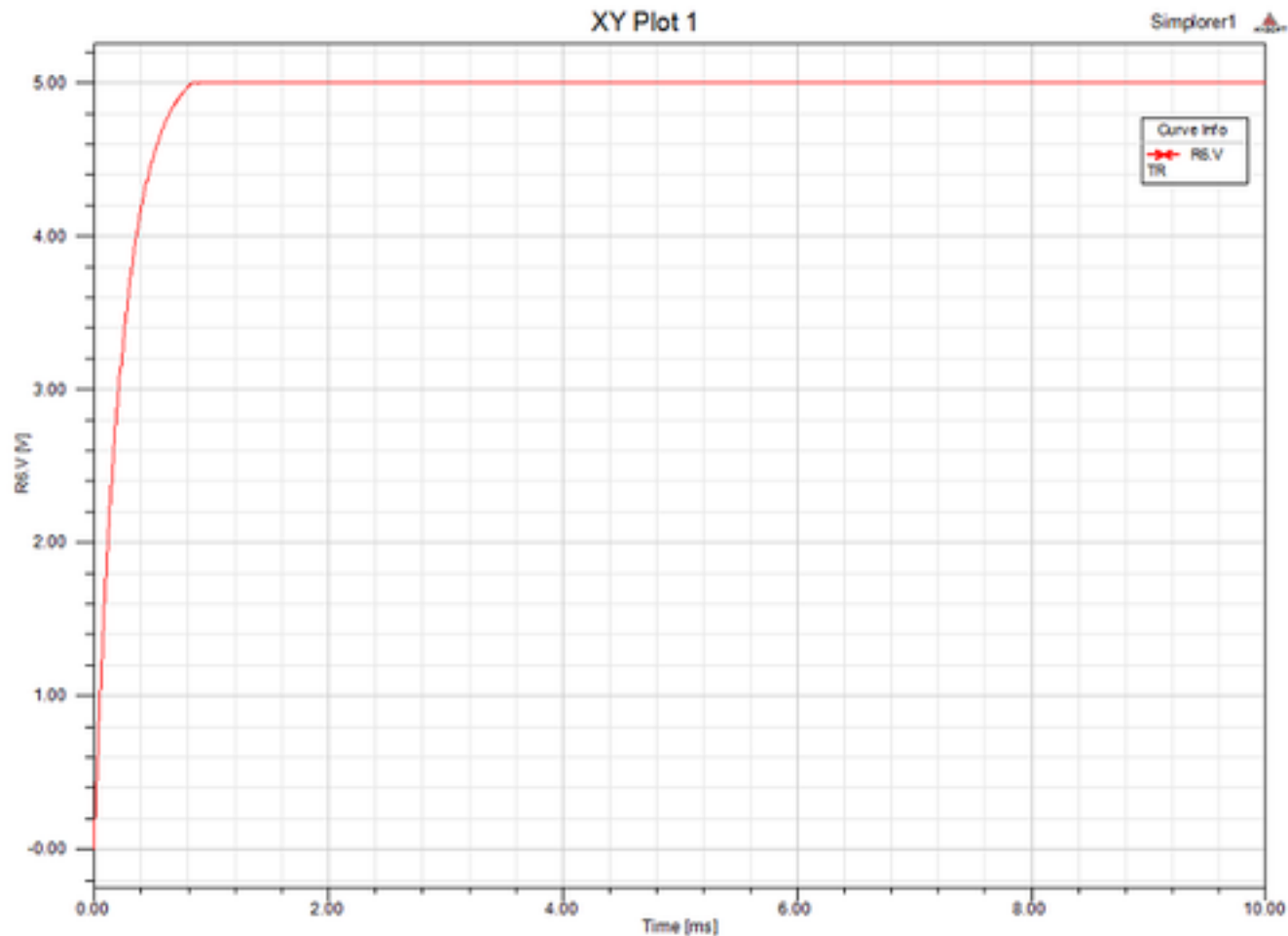
Figure 3. Simulation results
