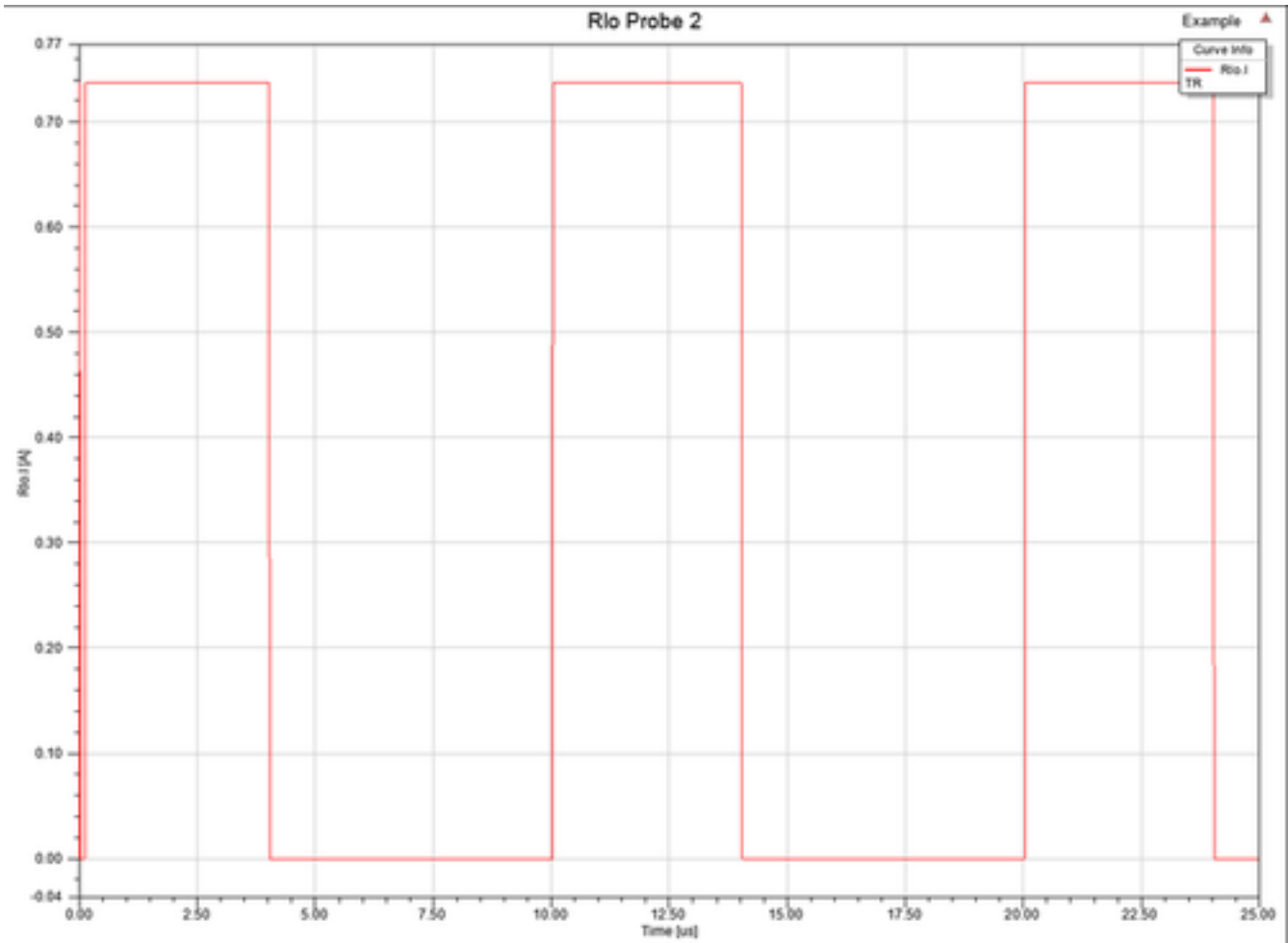
Figure 3. Simulation results
