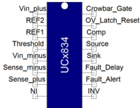
Figure 1. Component symbol
