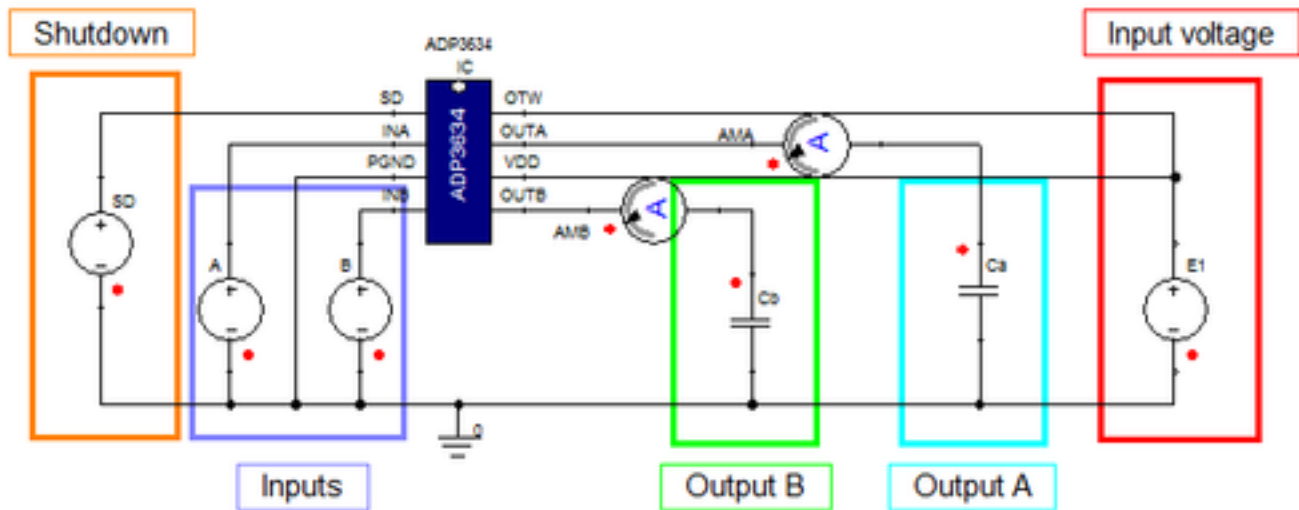
Figure 2. Example Circuit
