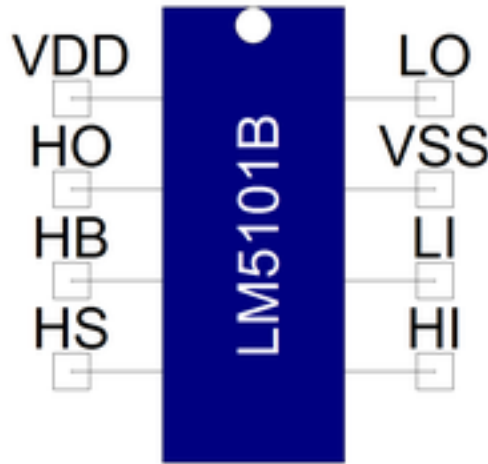
Figure 1. Component symbol
