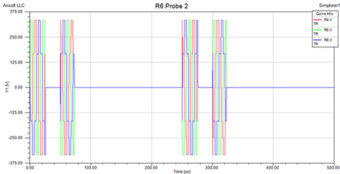
Figure 6. Protect Operation results(b)
