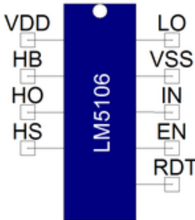
Figure 1. Component symbol
