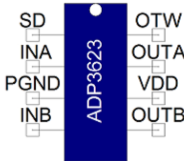
Figure 1. Component symbol
