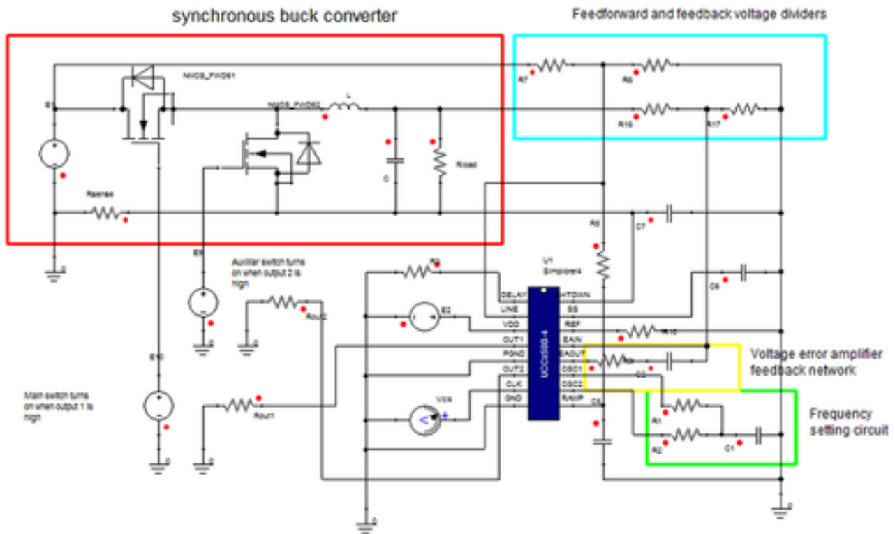
Figure 2. Example Circuit
