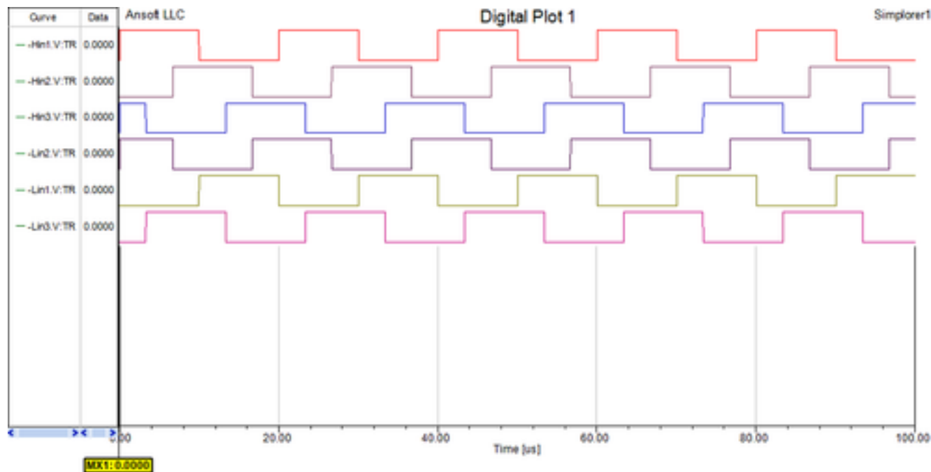
Figure 4. Main Operation results(b)
