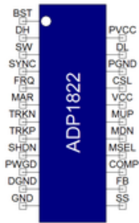
Figure 1. Component symbol
