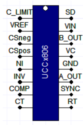
Figure 1. Component symbol
