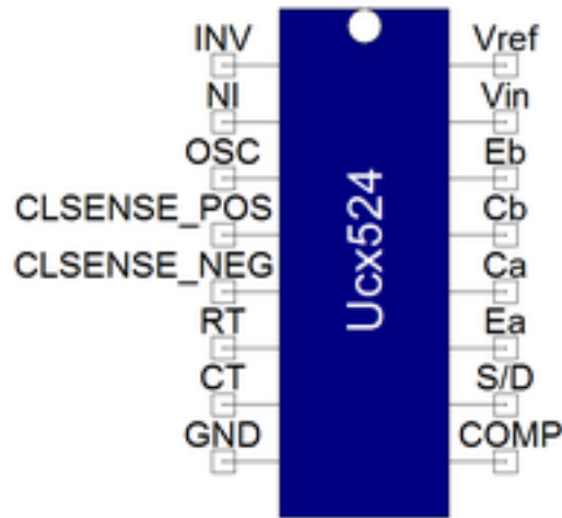
Figure 1. Component symbol
