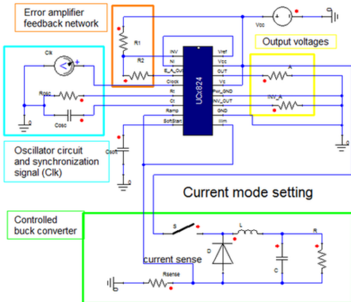
Figure 2. Example Circuit
