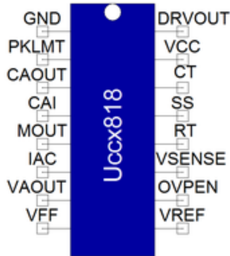
Figure 1. Component symbol
