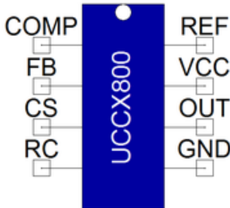
Figure 1. Component symbol
