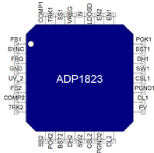
Figure 1. Component symbol
