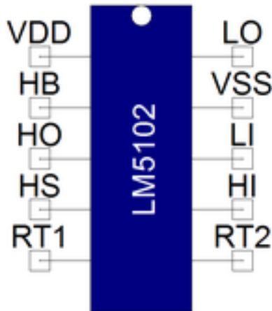
Figure 1. Component symbol
