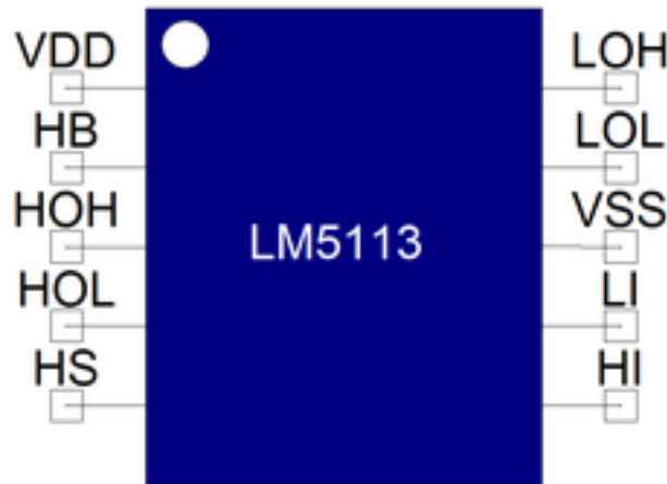
Figure 1. Component symbol
