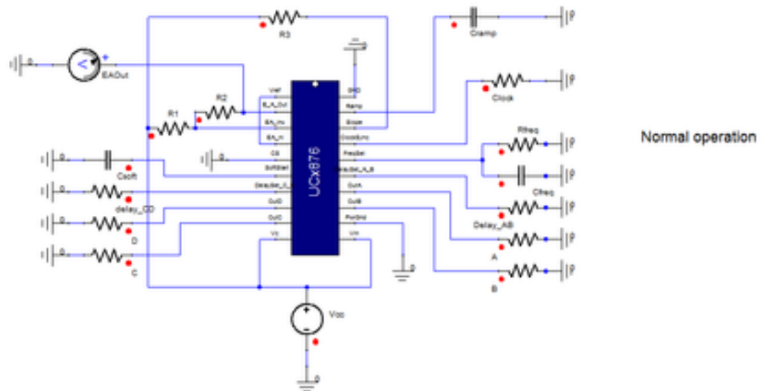
Figure 2. Example Circuit
