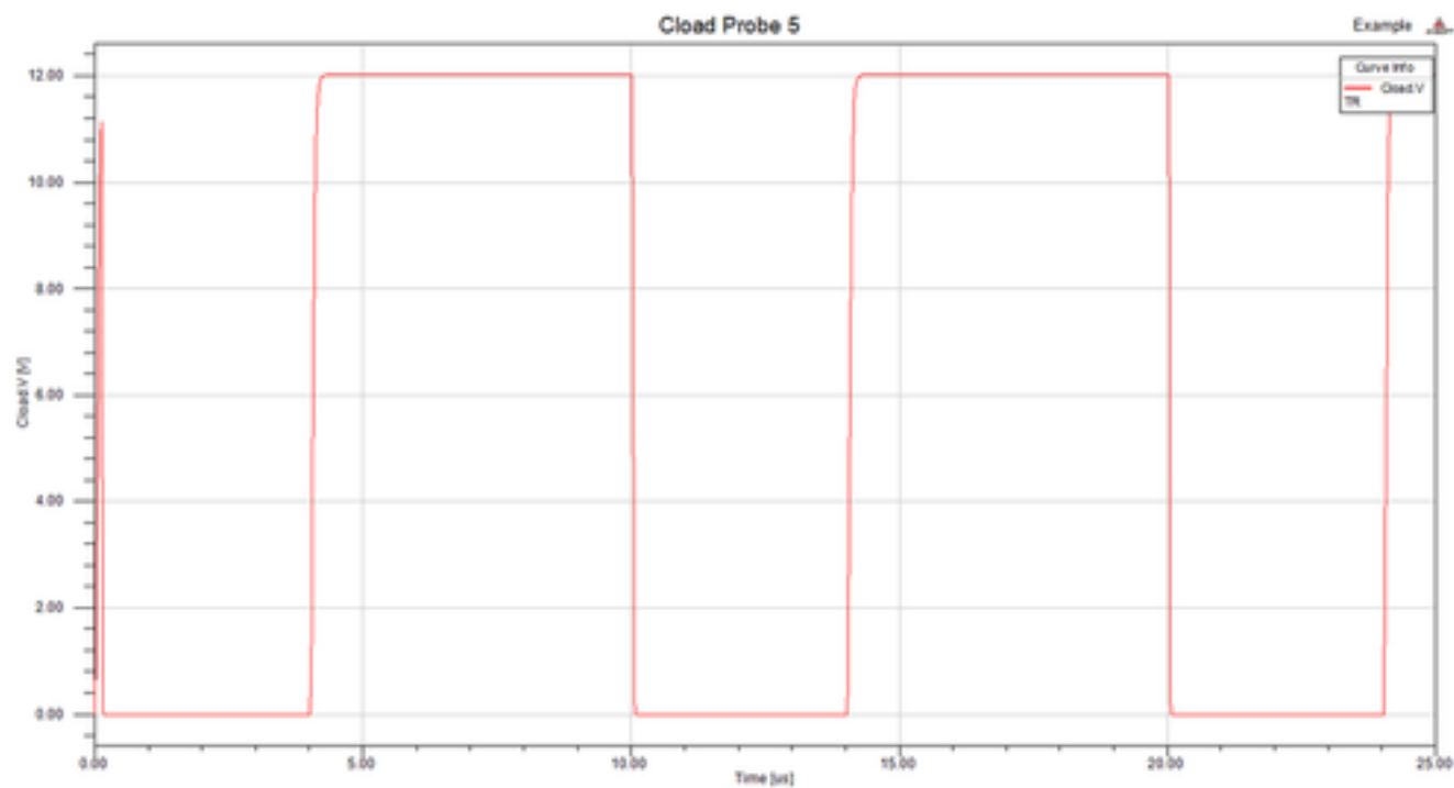
Figure 3. Simulation results
