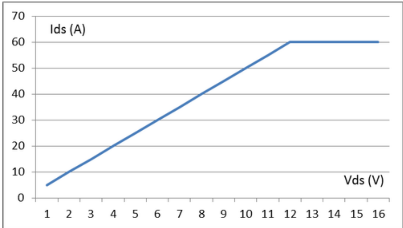
Figure 3. Conduction Resistance Curve
