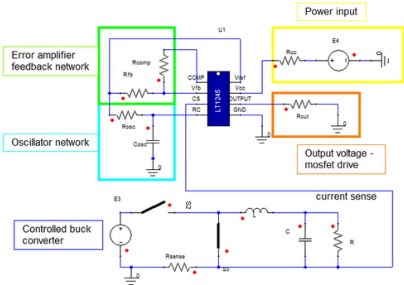
Figure 2. Example Circuit
