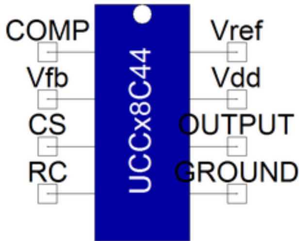
Figure 1. Component symbol
