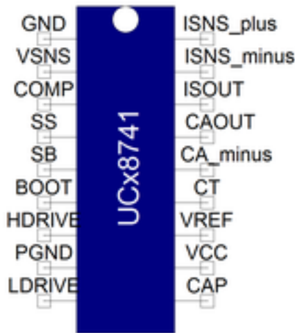
Figure 1. Component symbol
