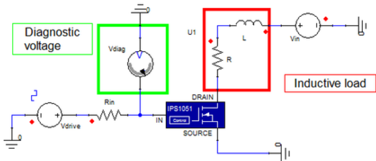
Figure 2. Example Circuit
