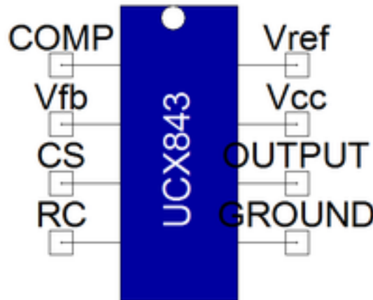
Figure 1. Component symbol
