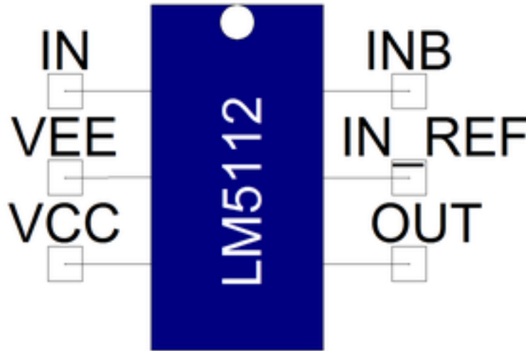
Figure 1. Component symbol
