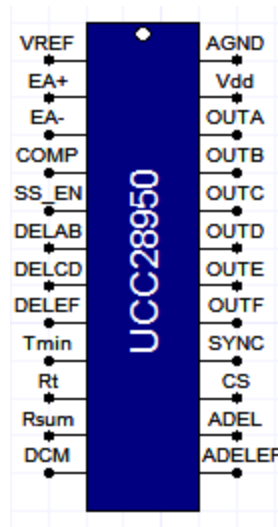
Figure 1. Component symbol
