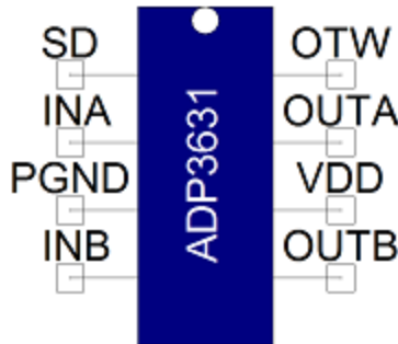
Figure 1. Component symbol
