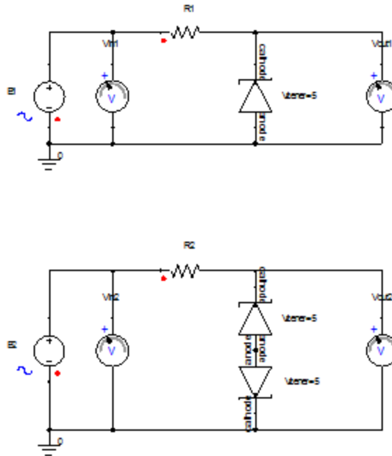
Figure 2. Application example of the System-Level Diode model
