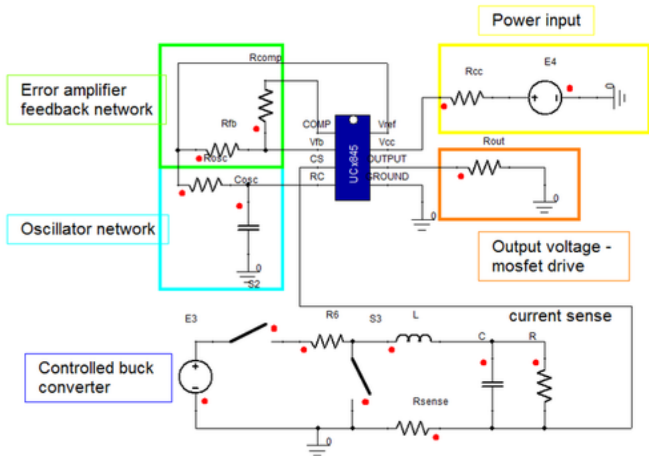
Figure 2. Example Circuit
