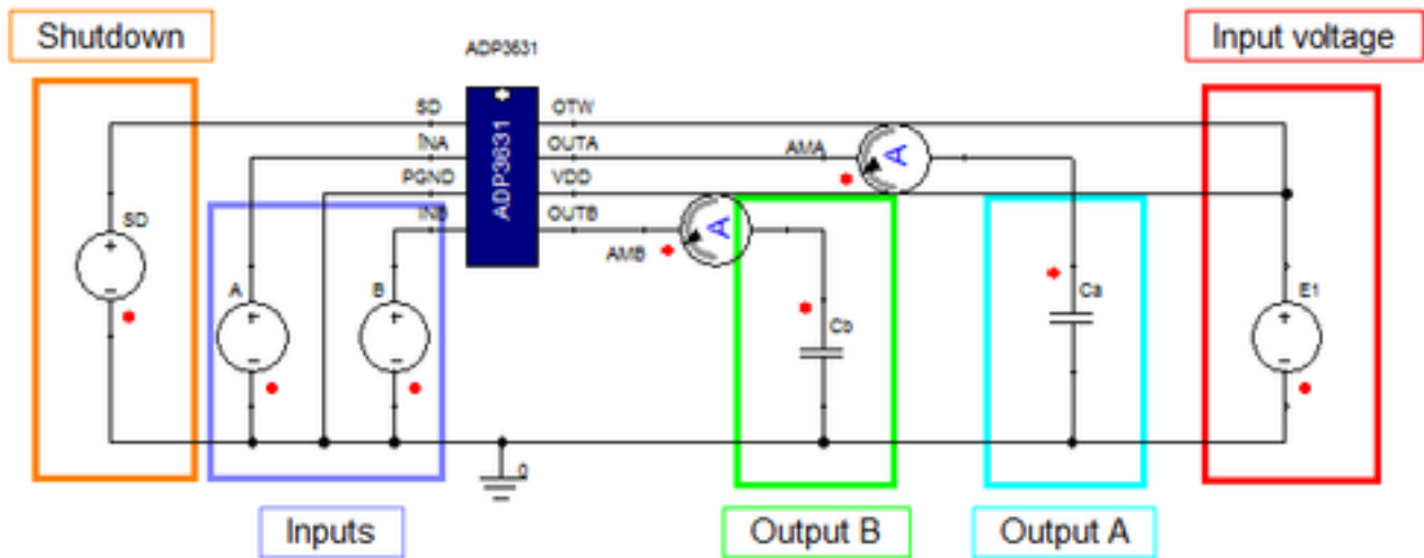
Figure 2. Example Circuit
