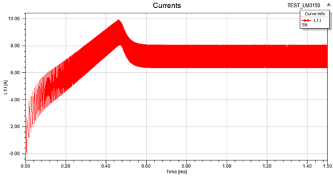
Figure 3. Inductor Current
