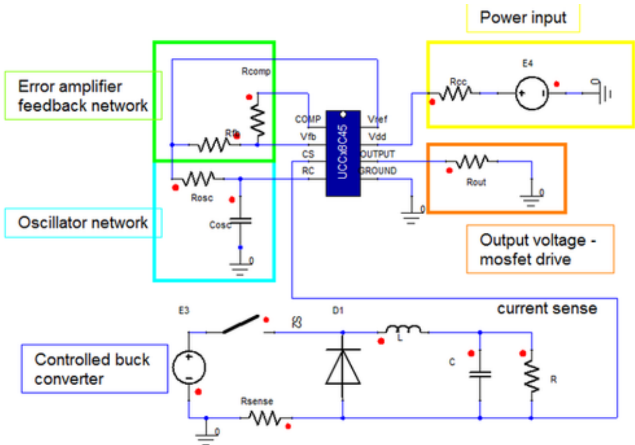
Figure 2. Example Circuit
