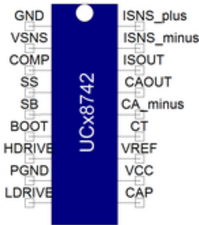
Figure 1. Component symbol
