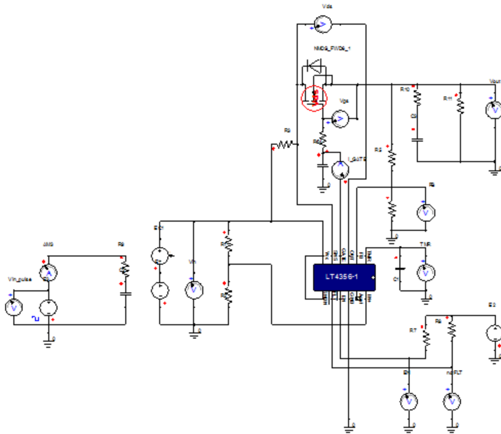
Figure 2. Example connection 4A, 12V Overvoltage Output Regulator
