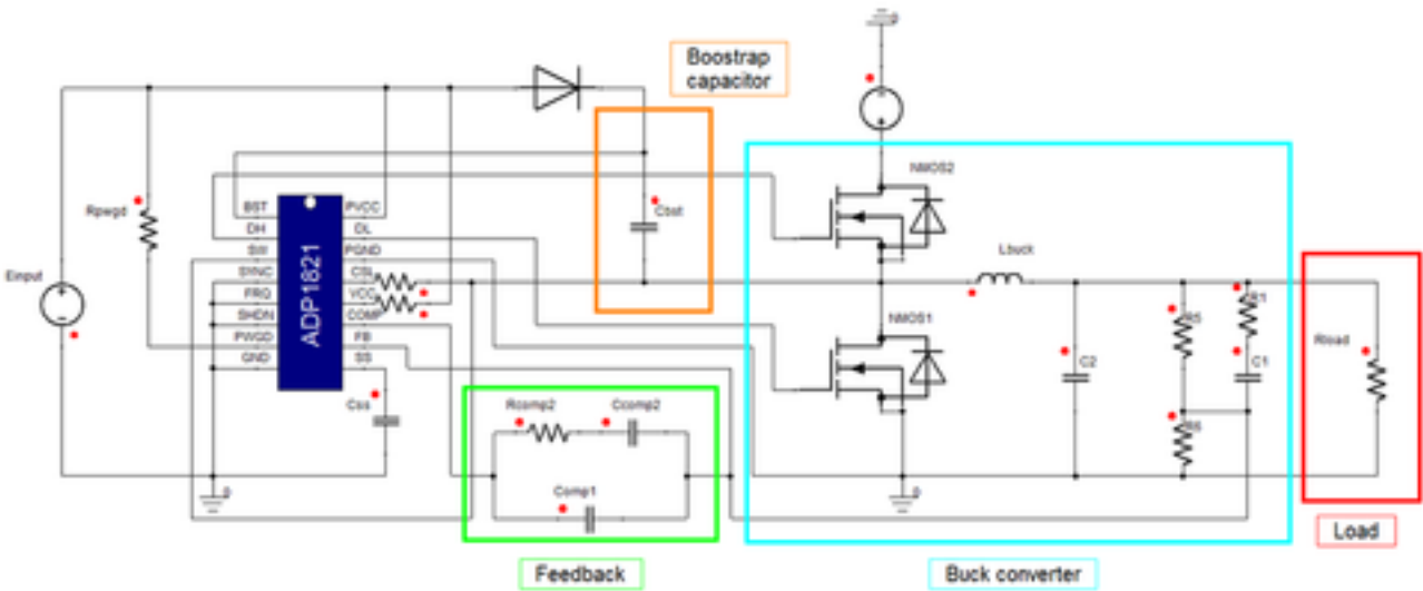
Figure 2. Example Circuit
