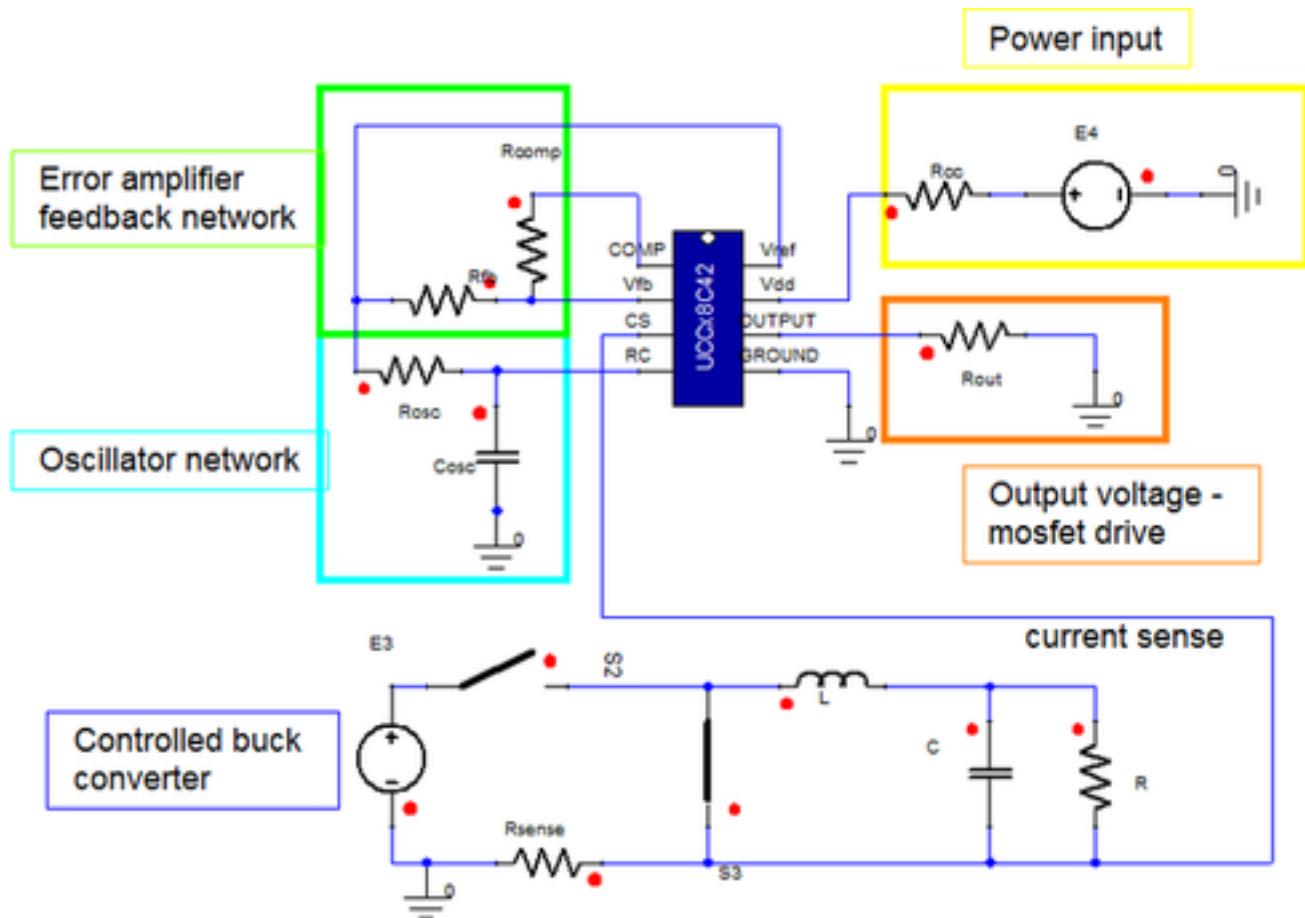
Figure 2. Example Circuit
