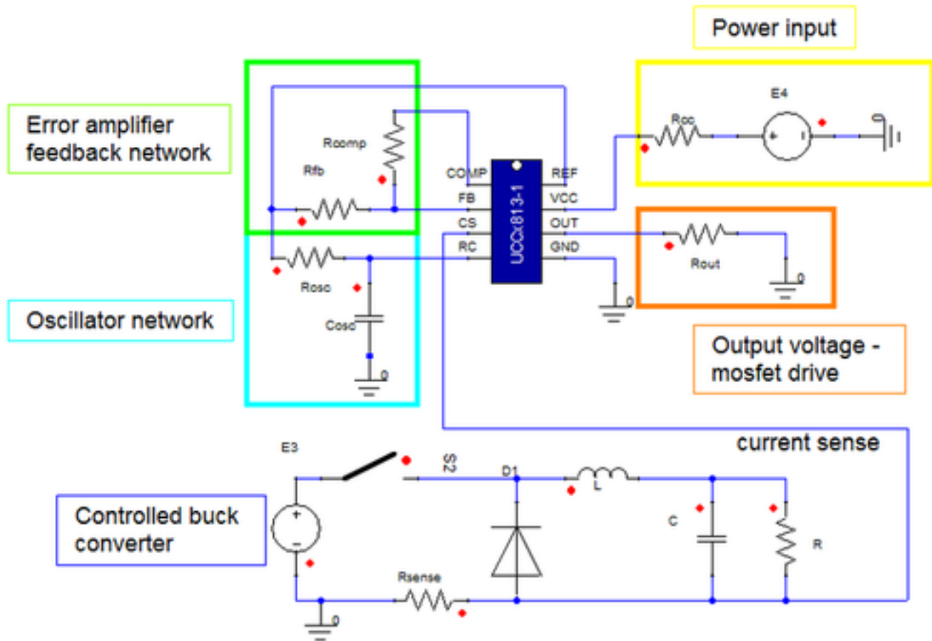
Figure 2. Example Circuit
