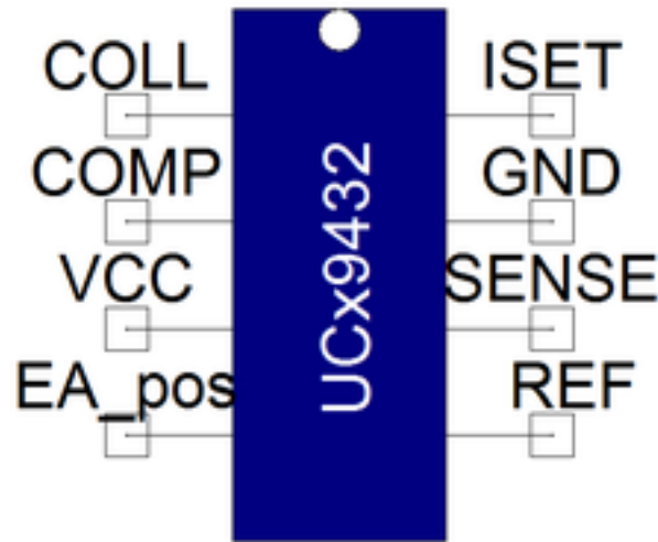
Figure 1. Component symbol
