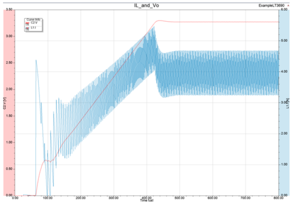
Figure 3. Waveforms
