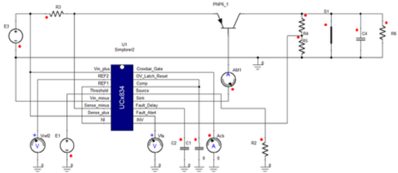
Figure 2. Example Circuit
