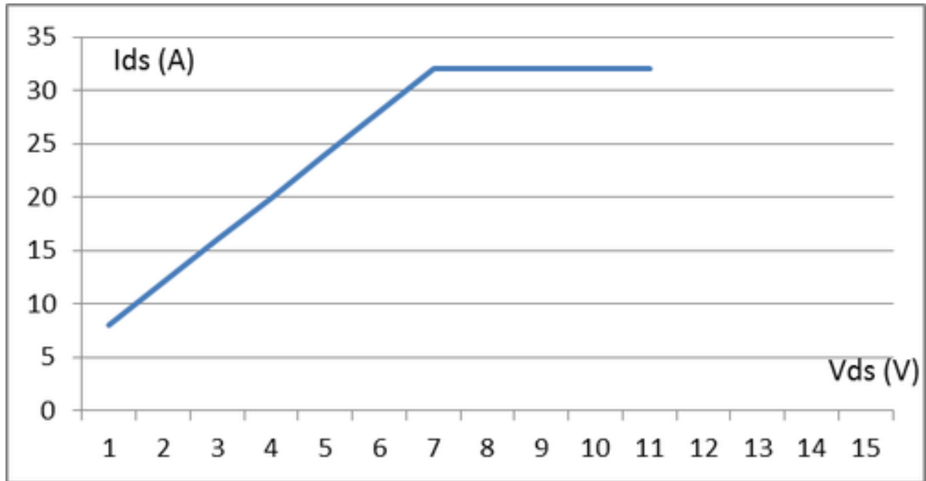
Figure 3. Conduction Resistance Curve
