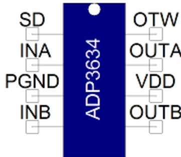
Figure 1. Component symbol
