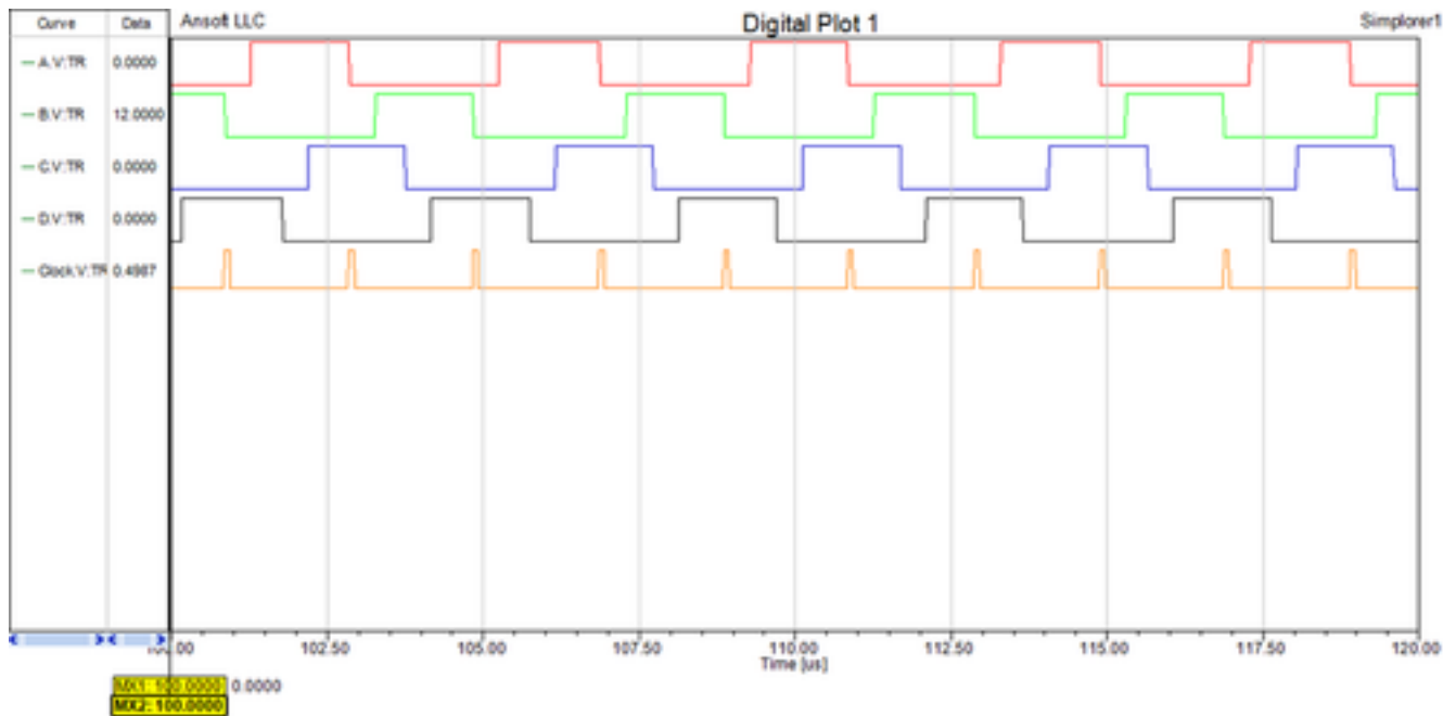
Figure 4 Simulation results(a)
