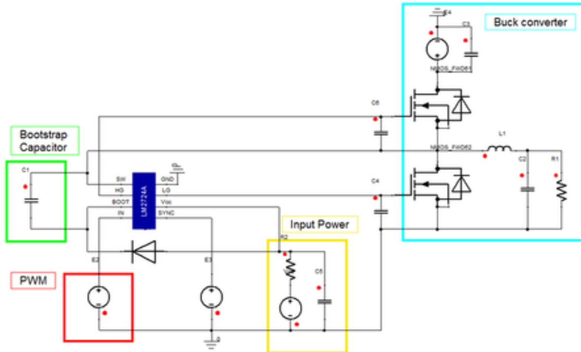
Figure 2. Example Circuit
