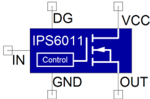
Figure 1. Component symbol
