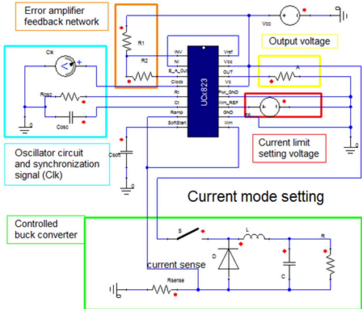
Figure 2. Example Circuit
