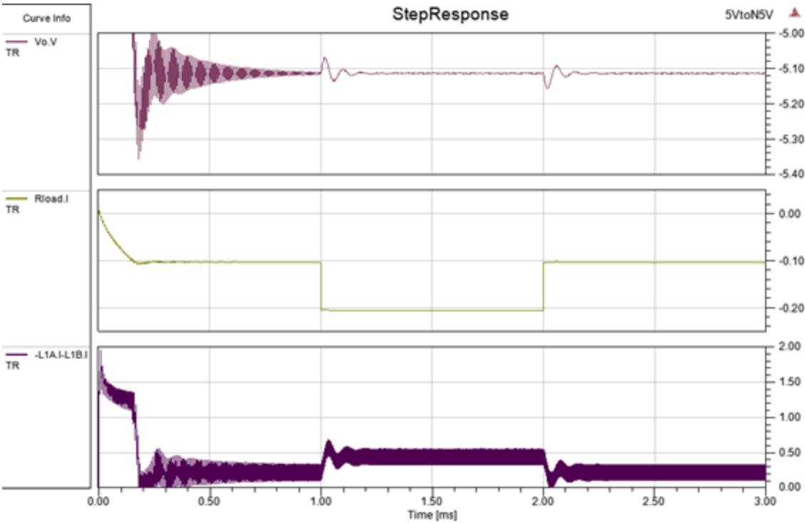
Figure 3. Step Response
