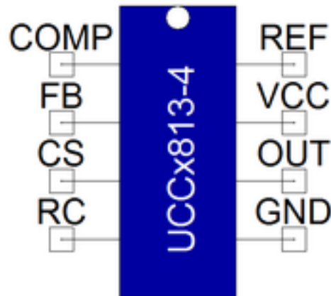
Figure 1. Component symbol
