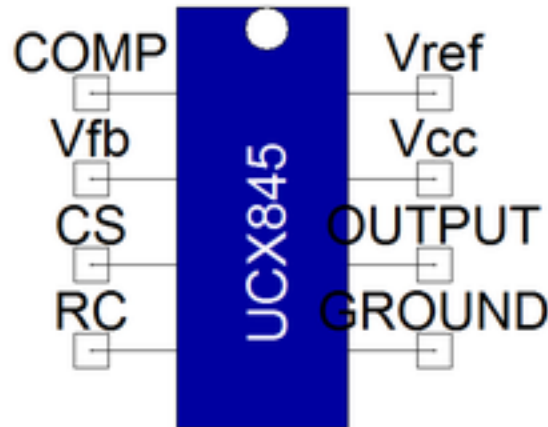
Figure 1. Component symbol
