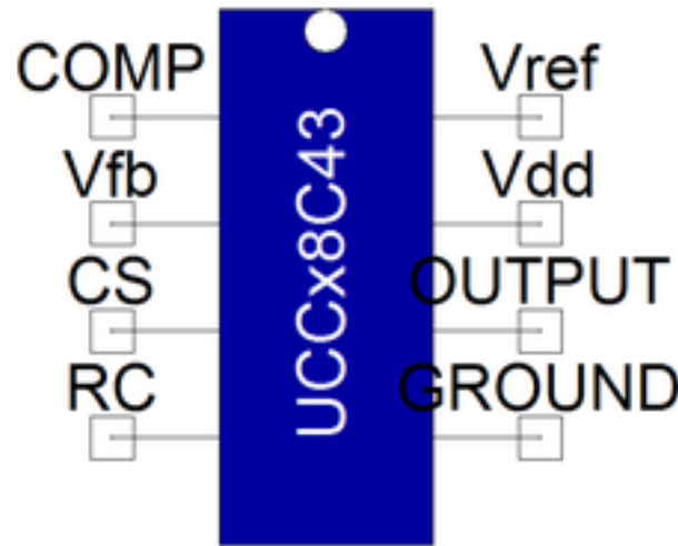
Figure 1. Component symbol
