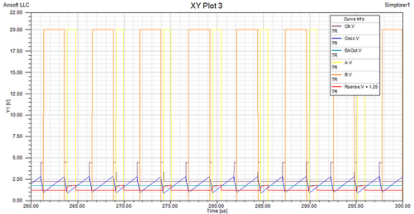
Figure 3. Simulation results(a)
