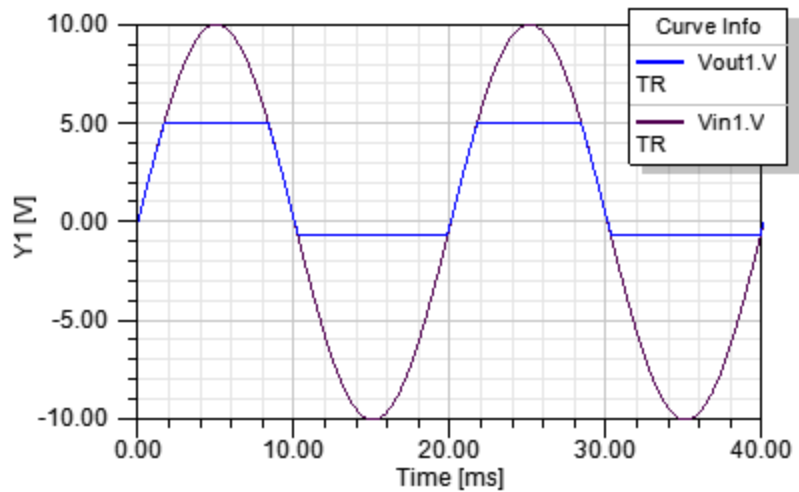
Figure 3. Simulation results for single Zener diode circuit
