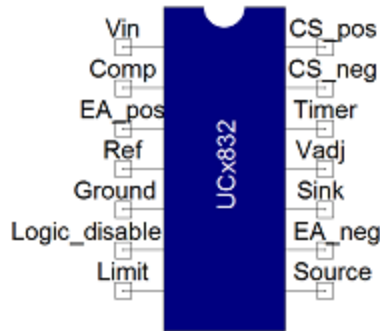
Figure 1. Component symbol
