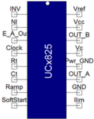
Figure 1. Component symbol
