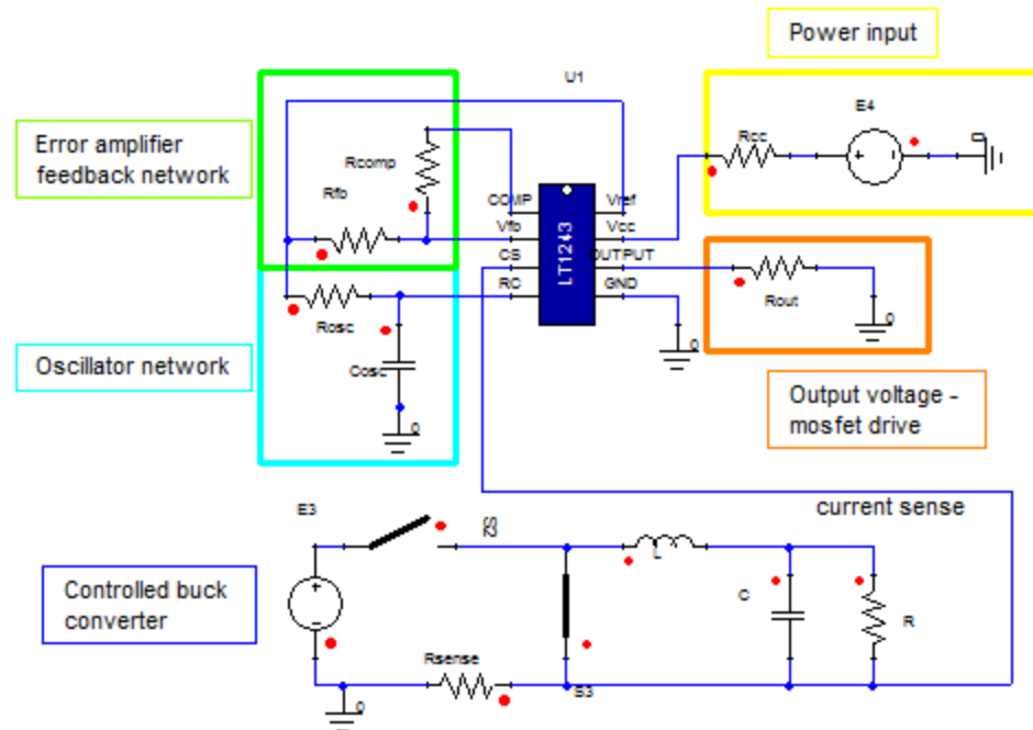
Figure 2. Example Circuit
