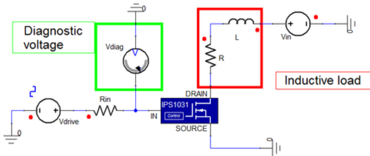
Figure 2. Example Circuit
