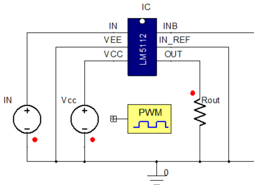
Figure 2. Example Circuit
