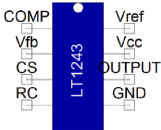
Figure 1. Component symbol
