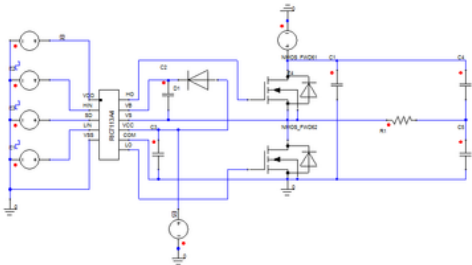
Figure 2. Example Circuit
