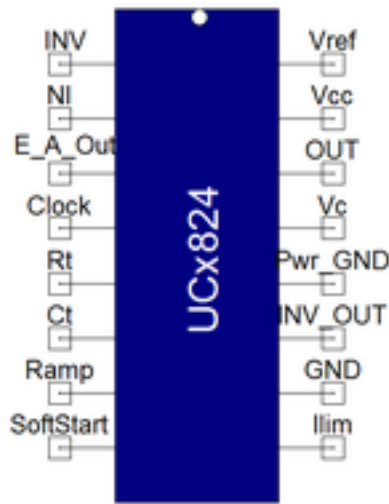
Figure 1. Component symbol
