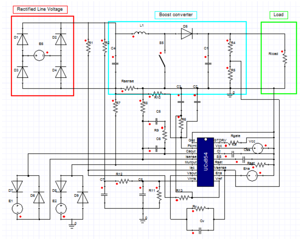
Figure 2. Example Circuit
