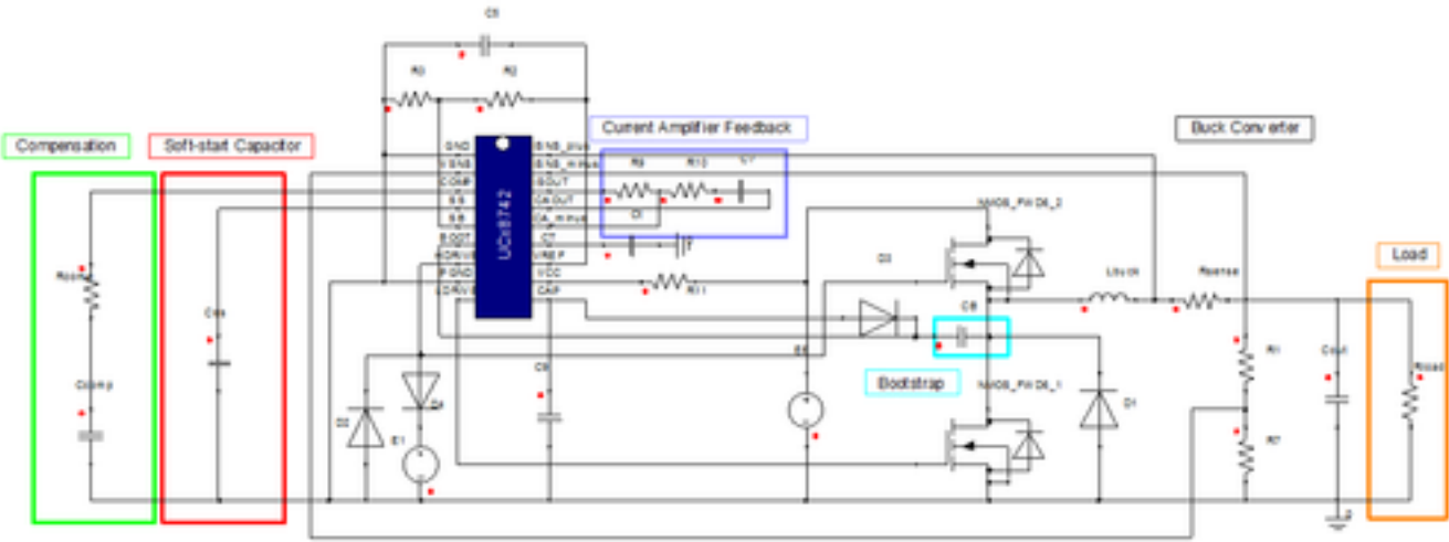
Figure 2. Example Circuit
