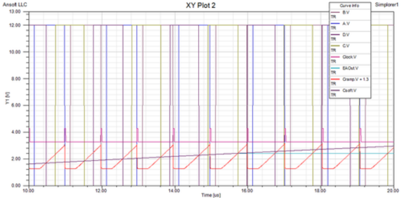
Figure 5. Simulation results(b)
