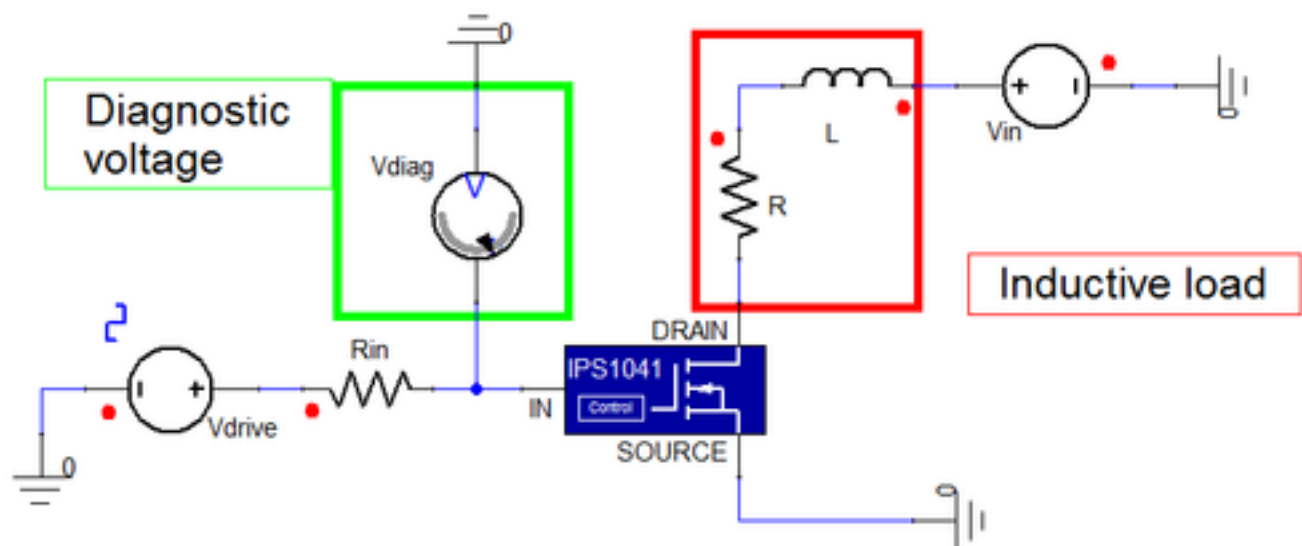
Figure 2. Example Circuit
