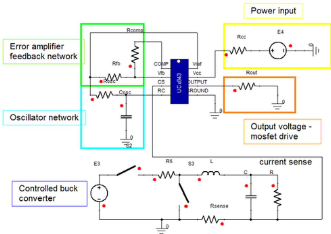
Figure 2. Example Circuit
