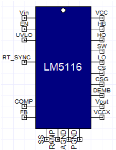
Figure 1. Component symbol
