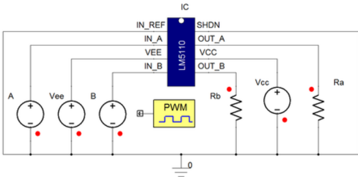
Figure 2. Example Circuit
