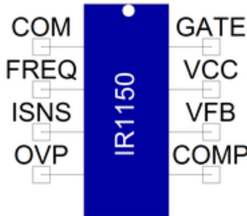
Figure 1. Component symbol
