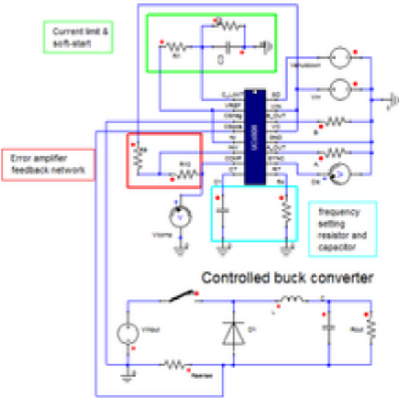
Figure 2. Example Circuit\
