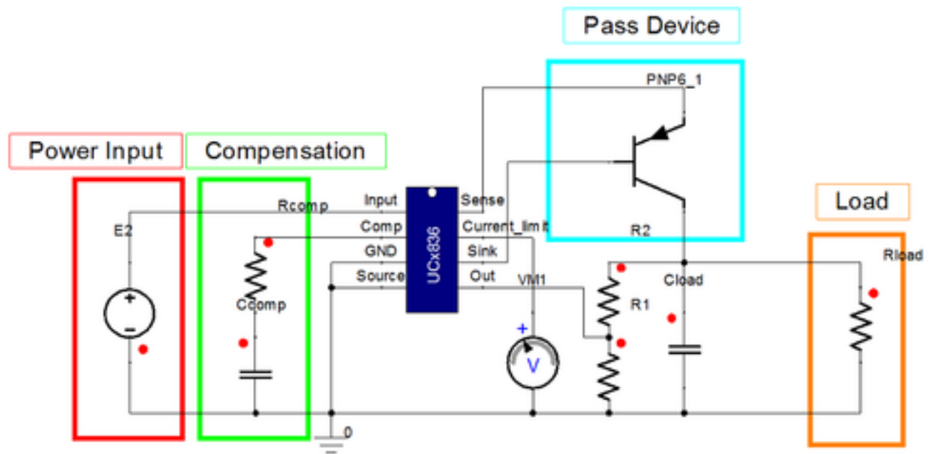
Figure 2. Example Circuit
