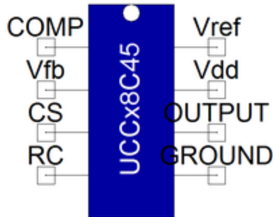
Figure 1. Component symbol
