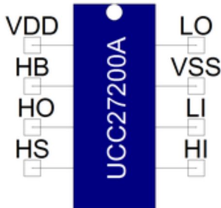
Figure 1. Component symbol
