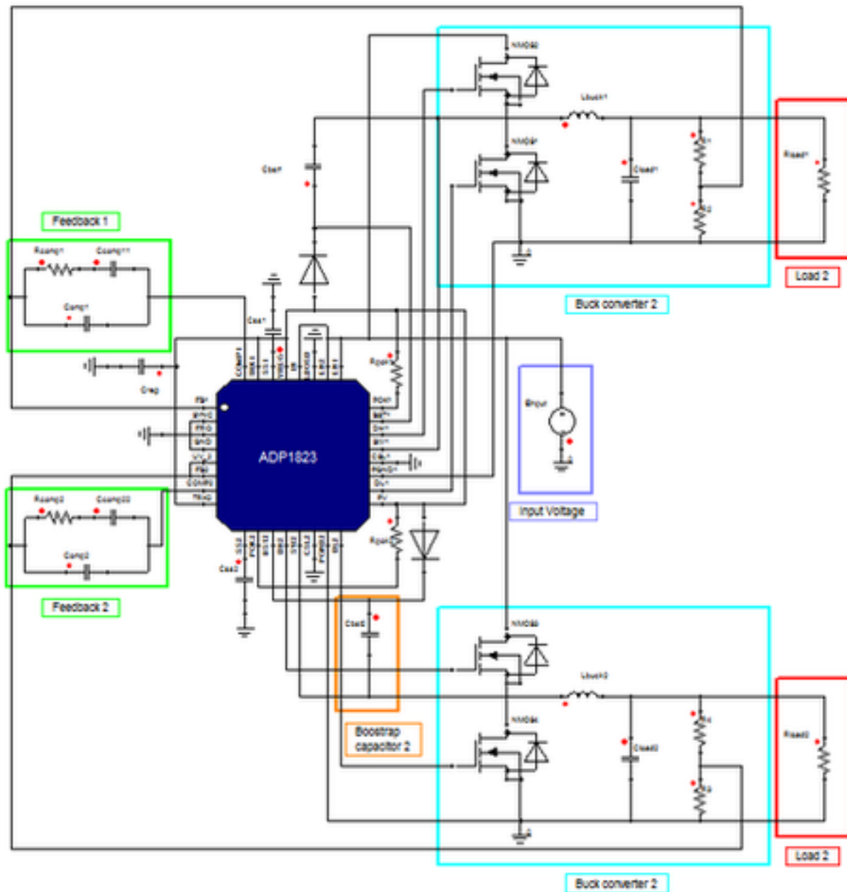
Figure 2. Example Circuit
