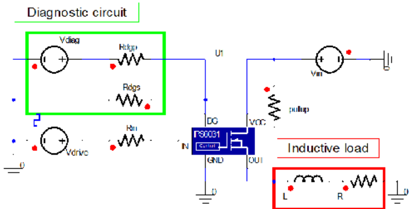
Figure 4. Example Circuit
