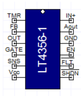
Figure 1. Component symbol
