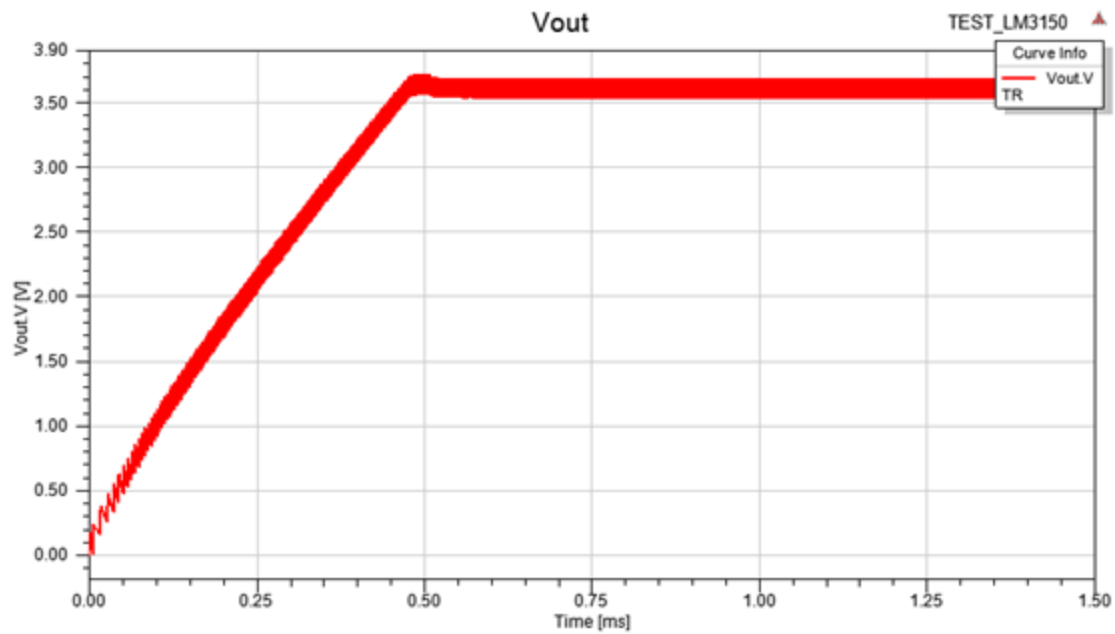
Figure 4: Output Voltage
