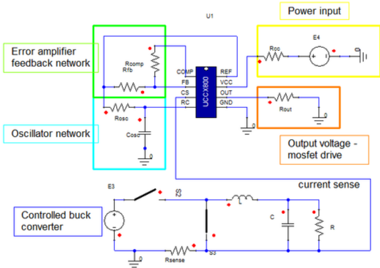
Figure 2. Example Circuit
