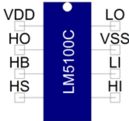
Figure 1. Component symbol
