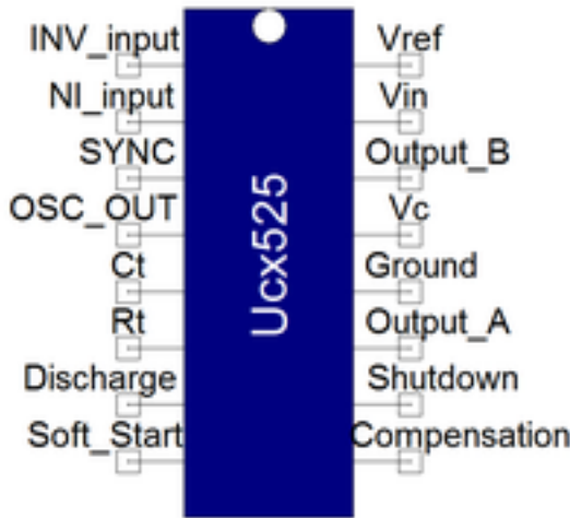
Figure 1. Component symbol
