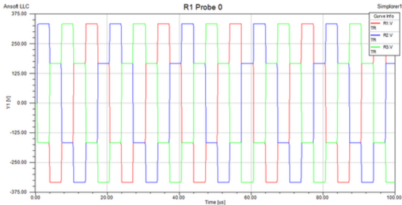
Figure 3. Main Operation results(a)
