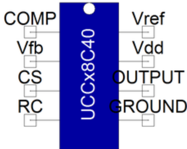
Figure 1. Component symbol
