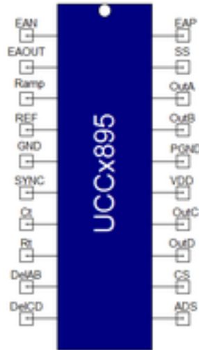
Figure 1. Component symbol
