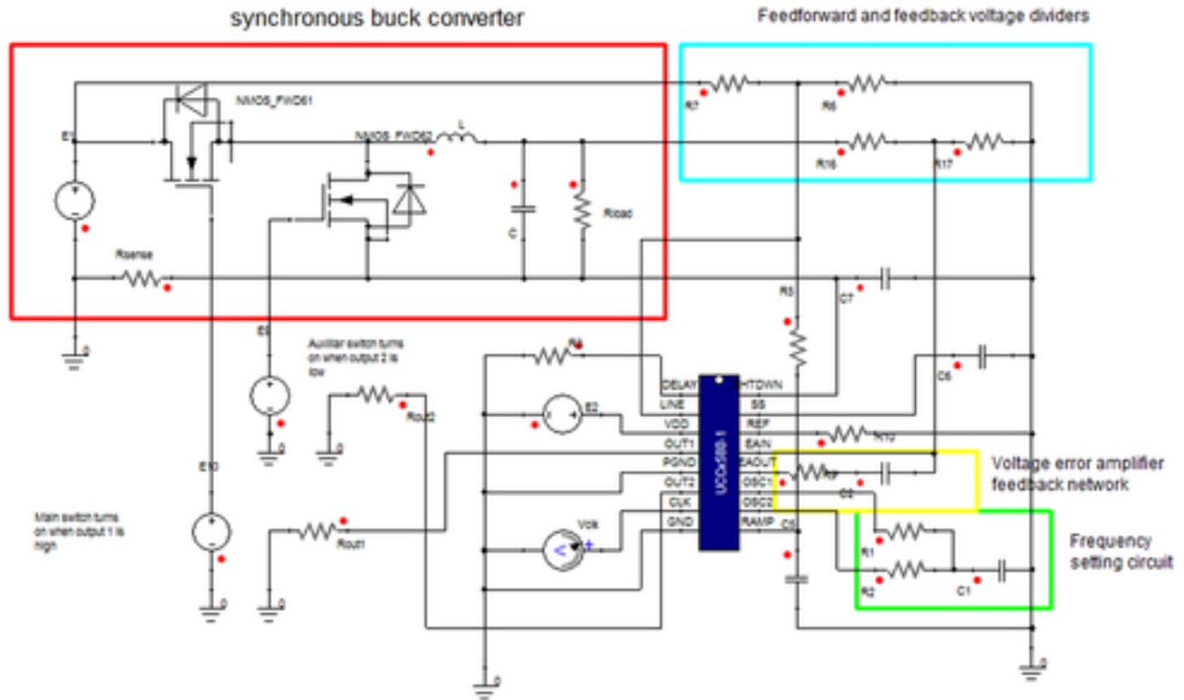
Figure 2. Example Circuit
