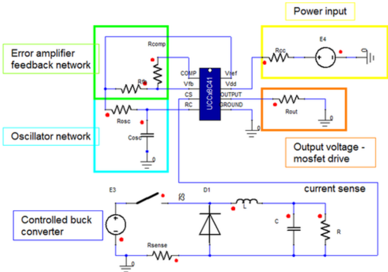
Figure 2. Example Circuit
