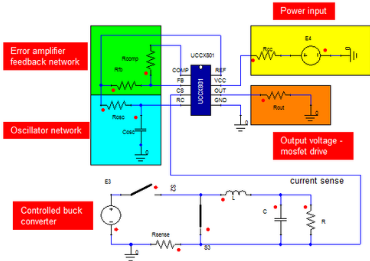
Figure 2. Example Circuit
