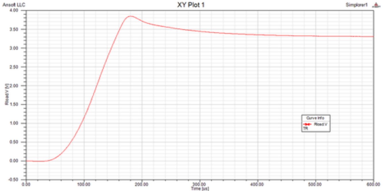
Figure 3. Simulation results(a)
