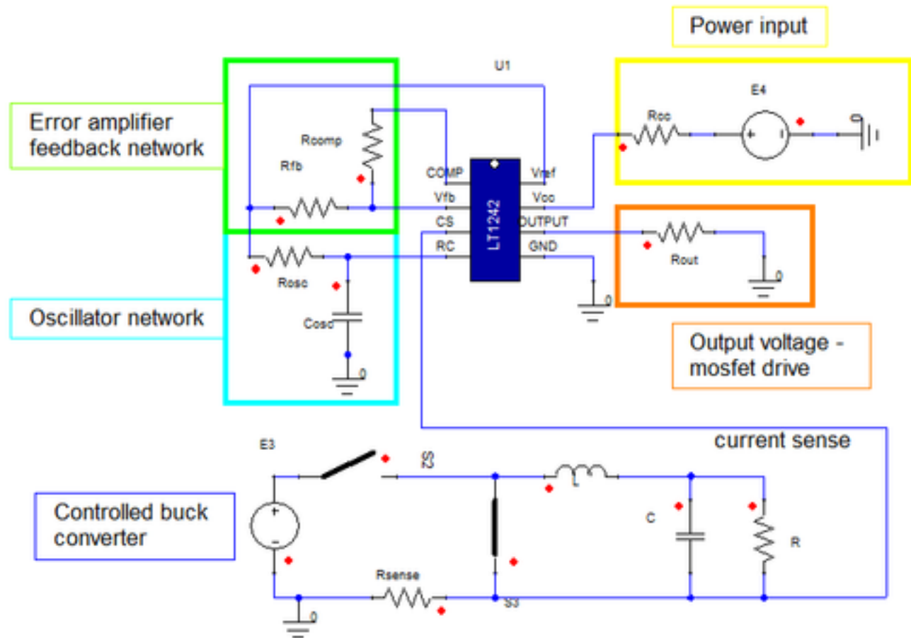
Figure 2. Example Circuit
