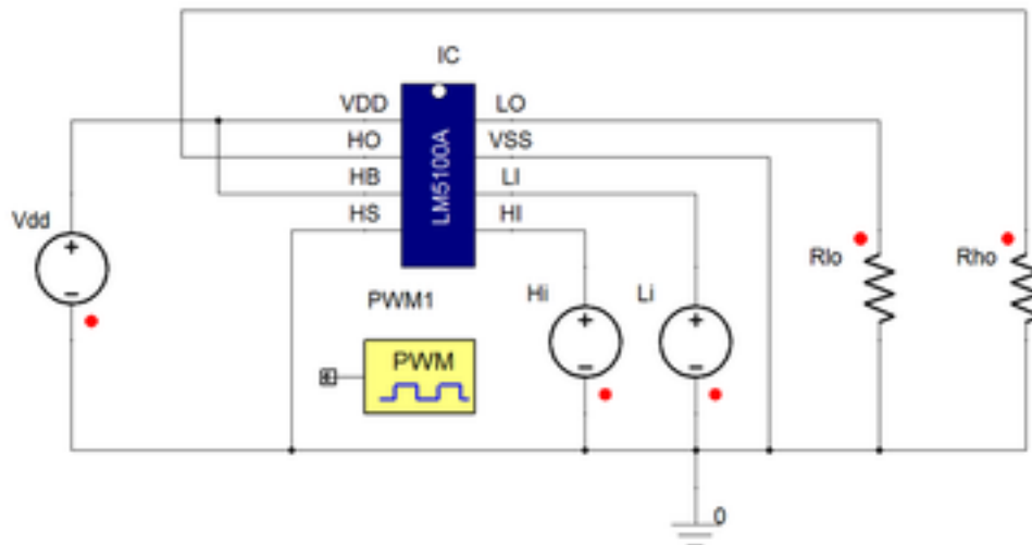
Figure 2. Example Circuit
