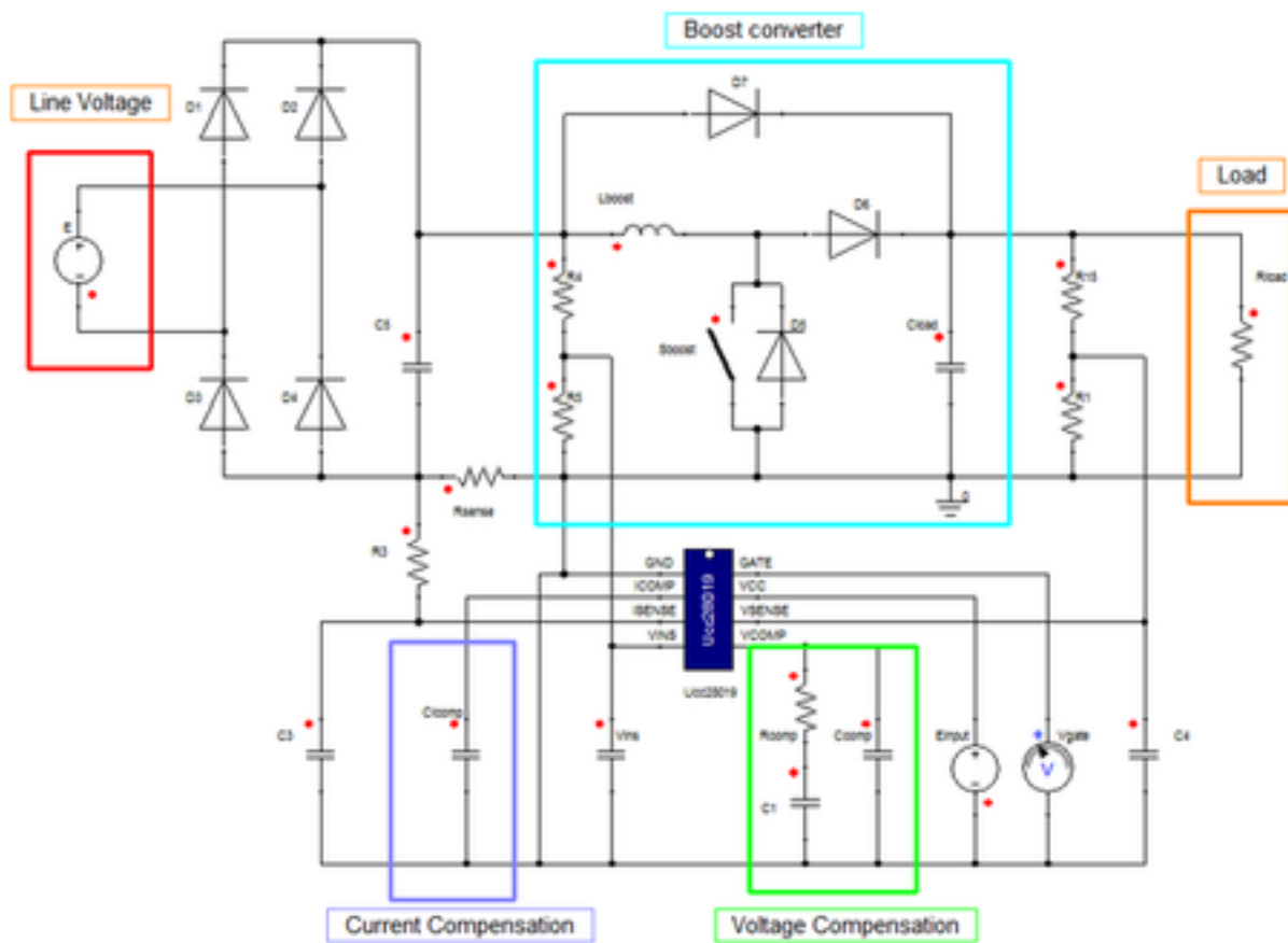
Figure 2. Example Circuit
