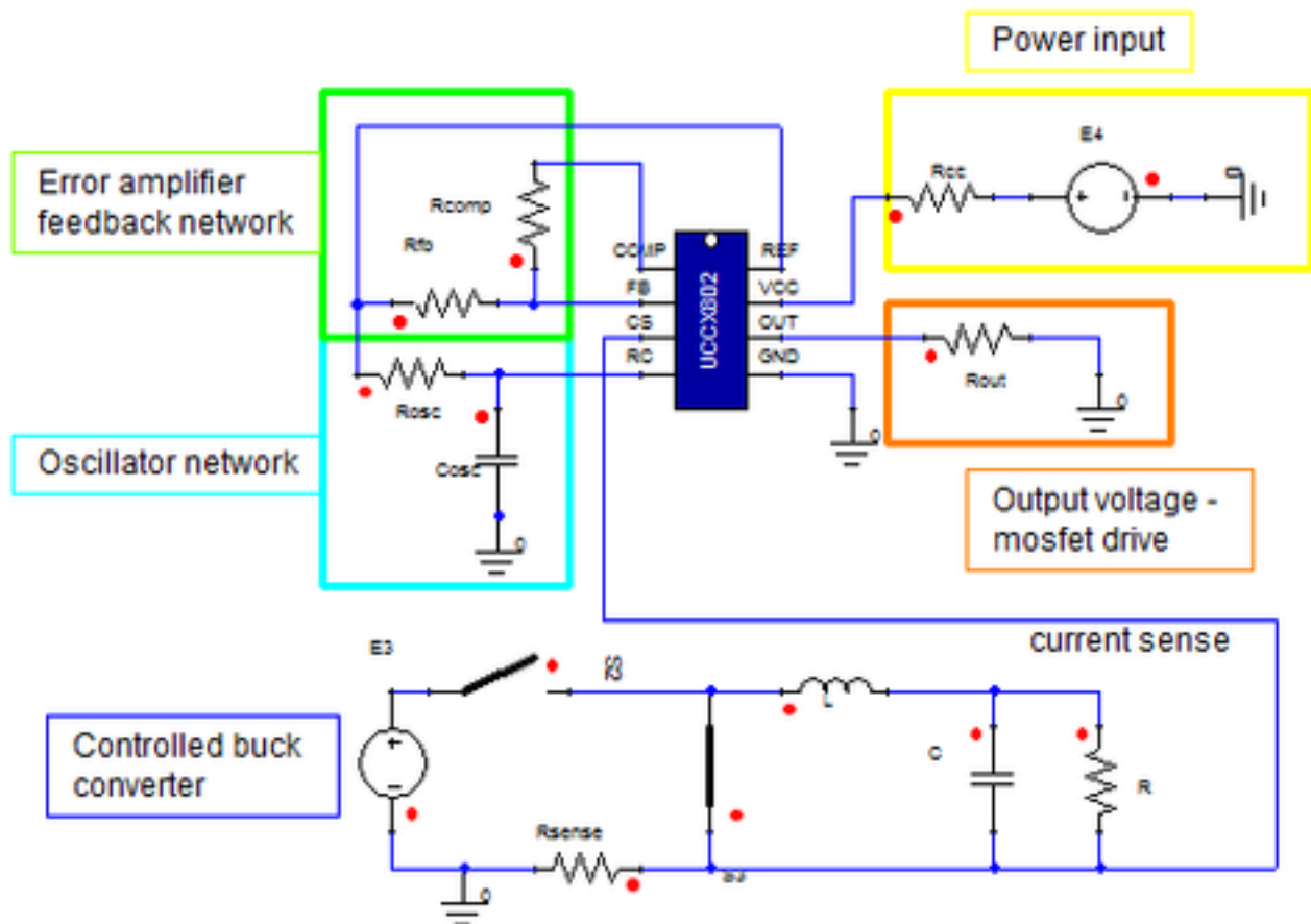
Figure 2. Example Circuit
