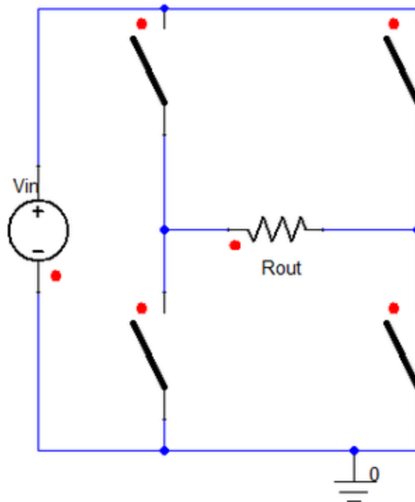
Figure 3. Four Switches Full-bridge Inverter
