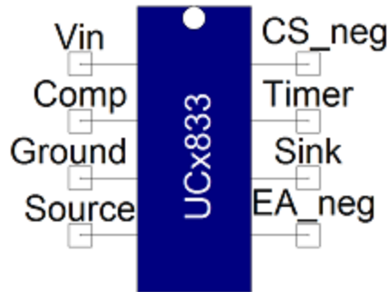
Figure 1. Component symbol
