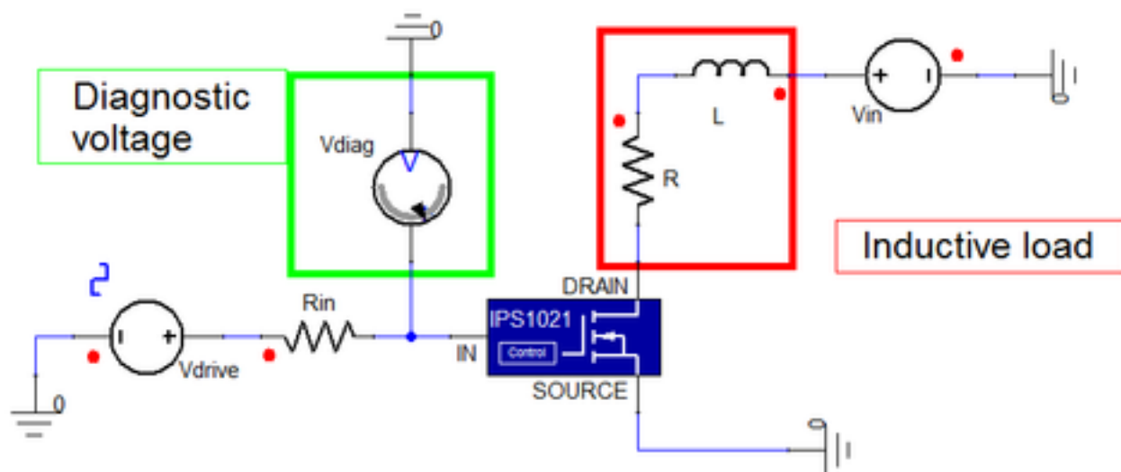
Figure 2. Example Circuit
