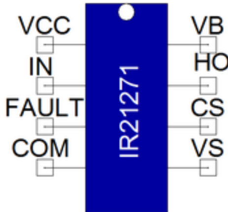
Figure 1. Component symbol
