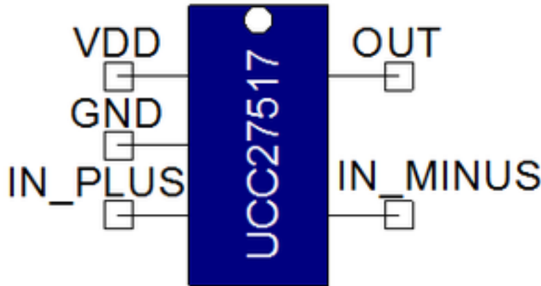
Figure 1. Component symbol
