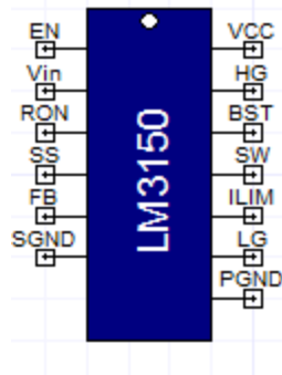
Figure 1. Component symbol
