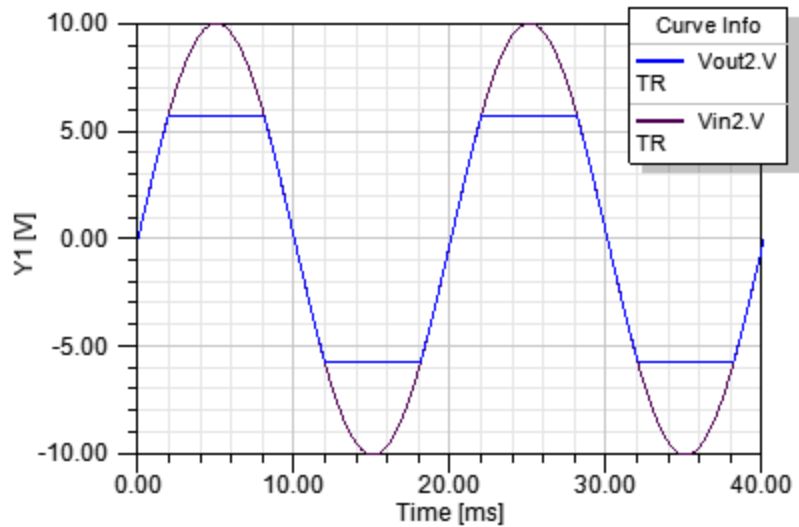
Figure 4. Simulation results for double Zener diode circuit
