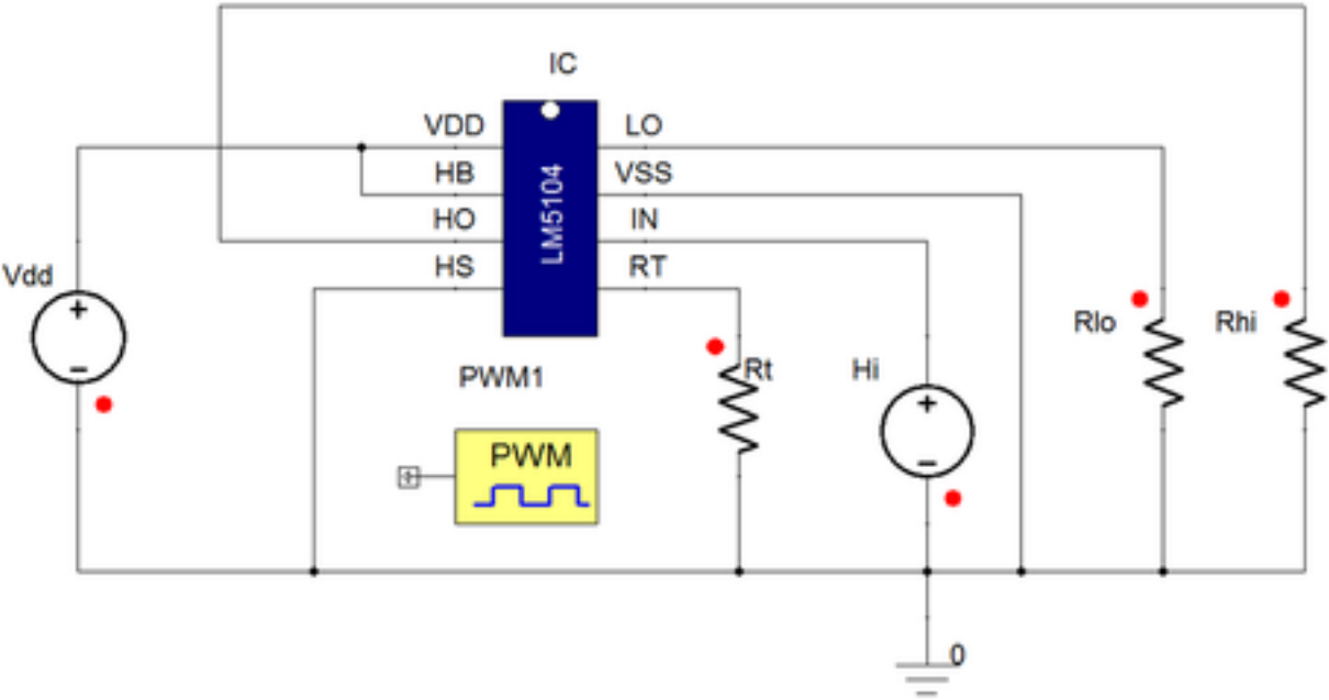
Figure 2. Example Circuit
