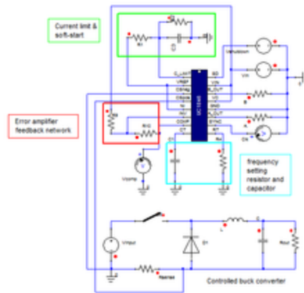
Figure 2. Example Circuit
