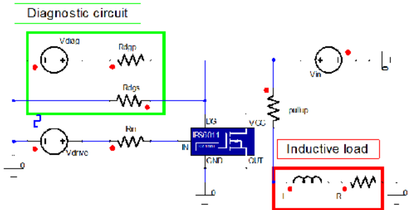
Figure 4. Example Circuit
