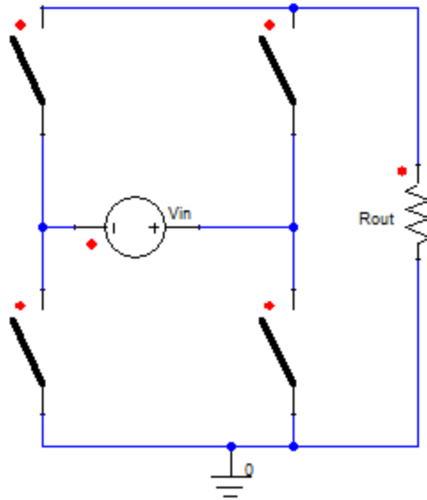
Figure 3. Four Switches Full-bridge Inverter
