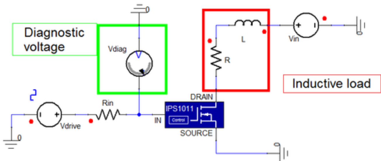
Figure 2. Example Circuit
