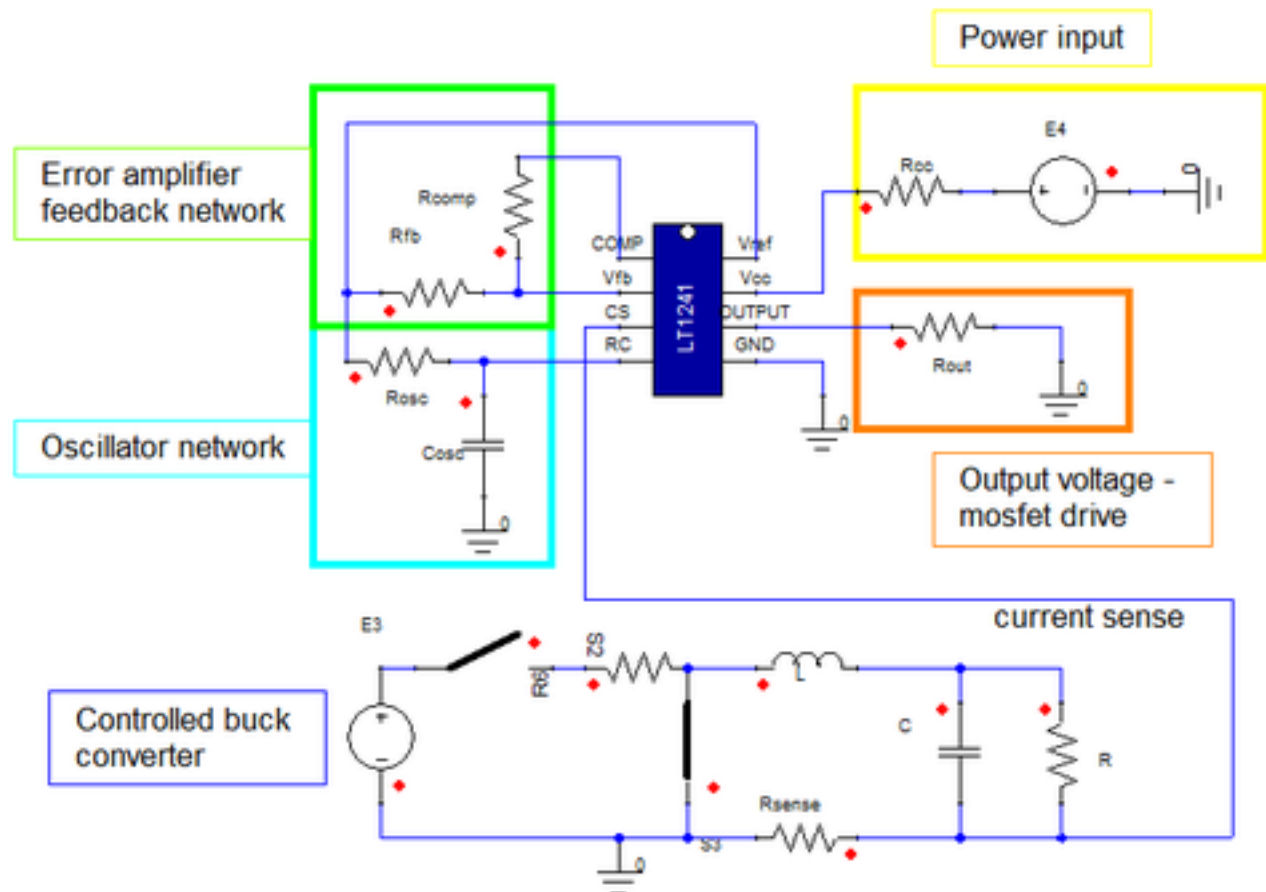
Figure 2. Example Circuit
