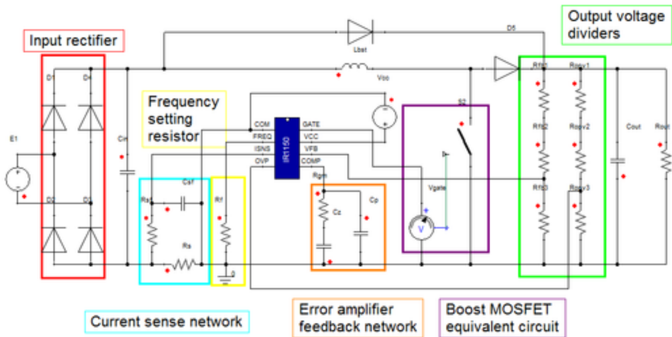
Figure 2. Example Circuit
