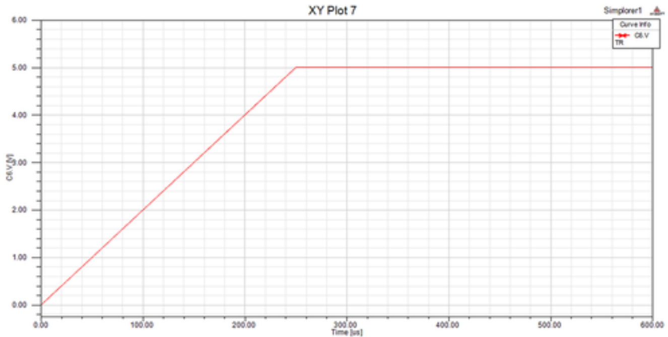
Figure 5. Simulation results(c)
