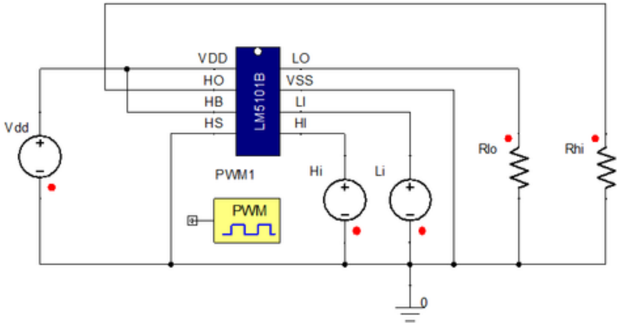
Figure 2. Example Circuit
