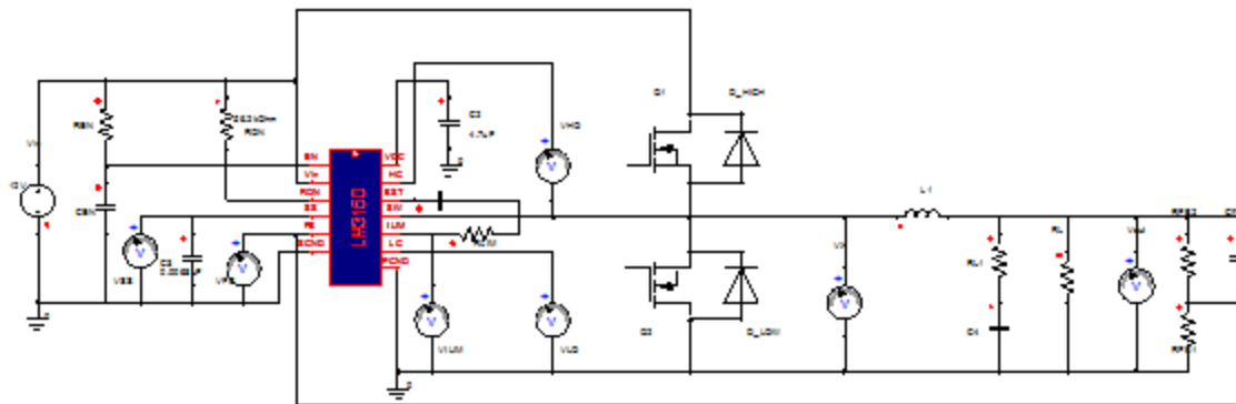
Figure 2. Twin Builder Schematic Example of use of the LM3150
