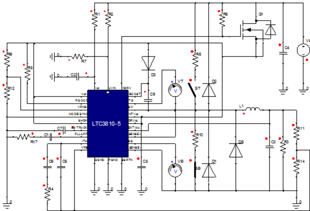
Figure 2. Example of Connection - 24V to 5V@6A
