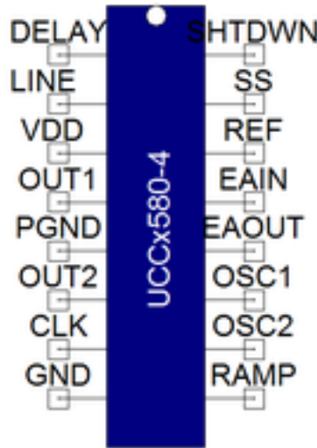
Figure 1. Component symbol
