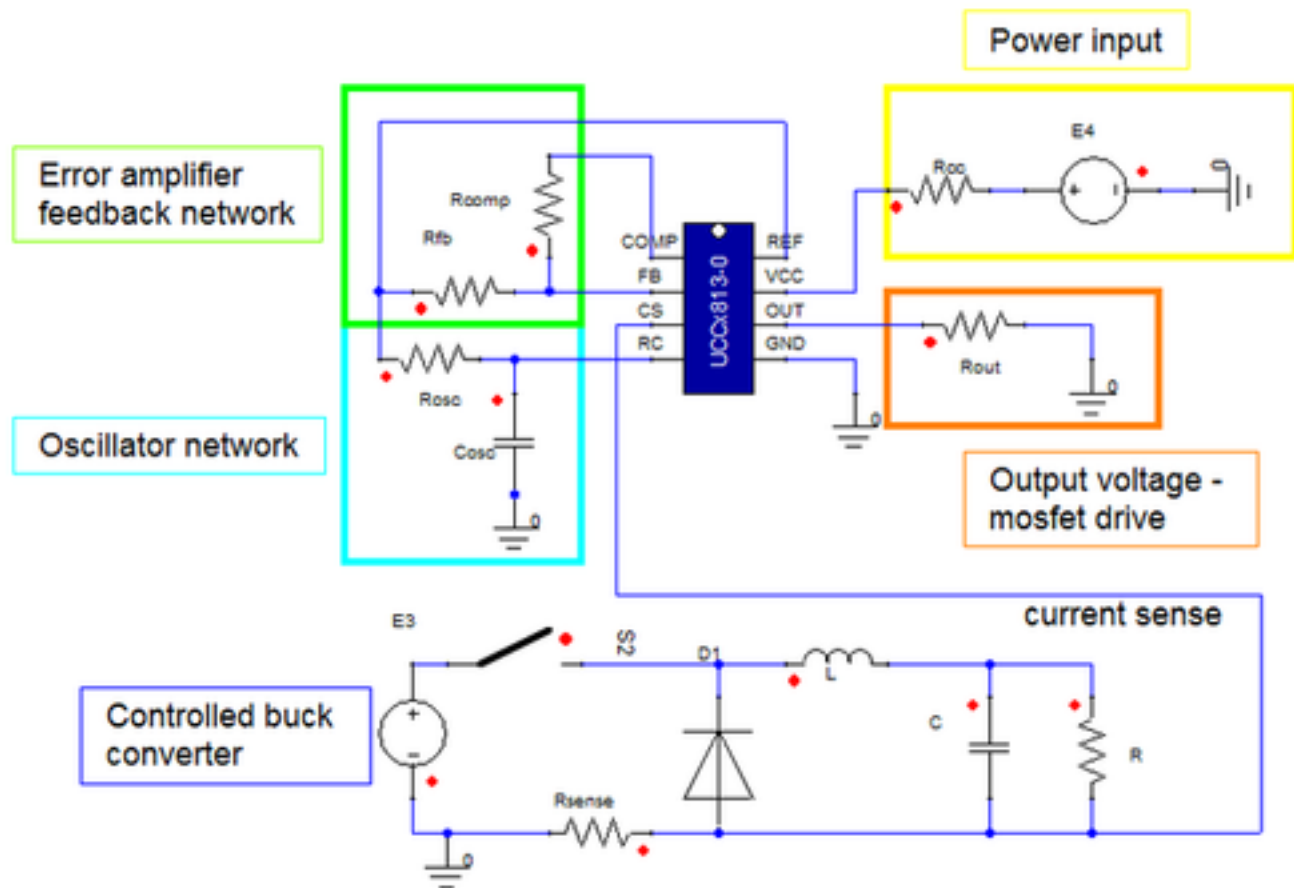
Figure 2. Example Circuit
