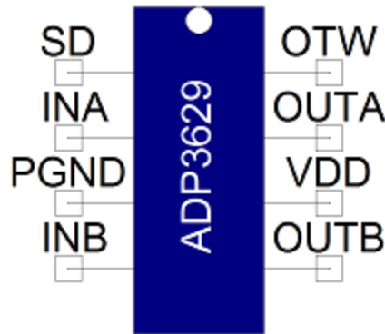
Figure 1. Component symbol
