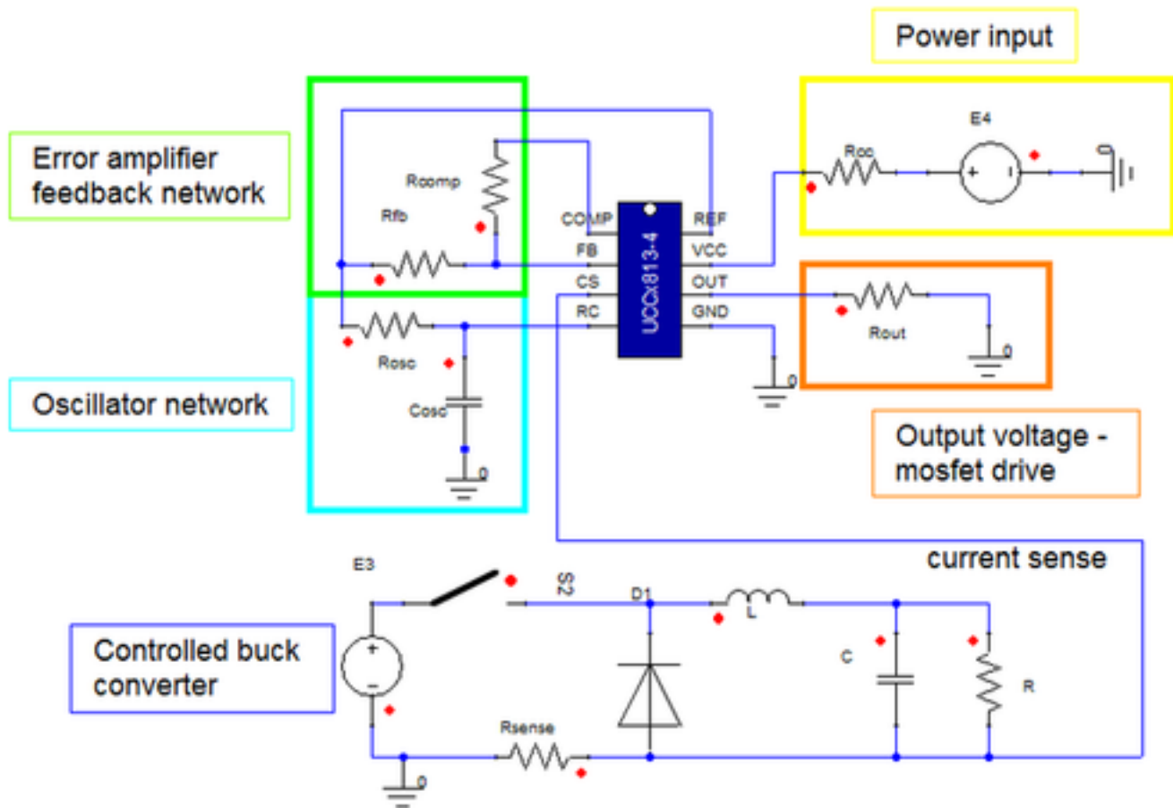
Figure 2. Example Circuit
