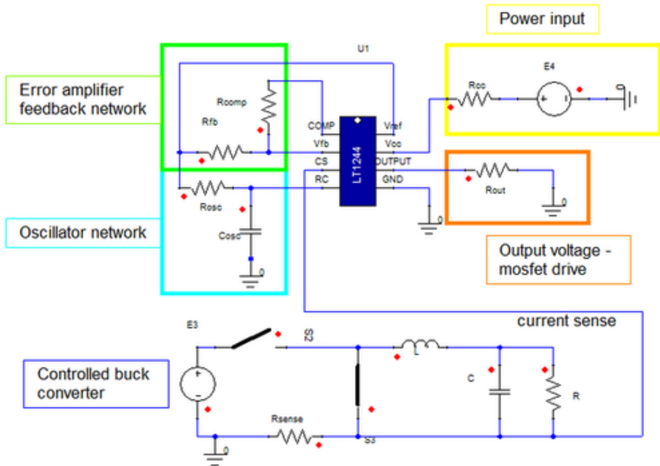
Figure 2. Example Circuit
