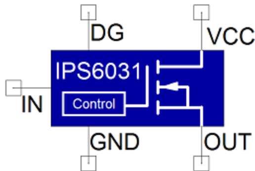
Figure 1. Component symbol
