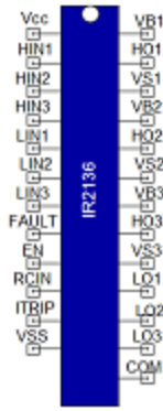
Figure 1. Component symbol
