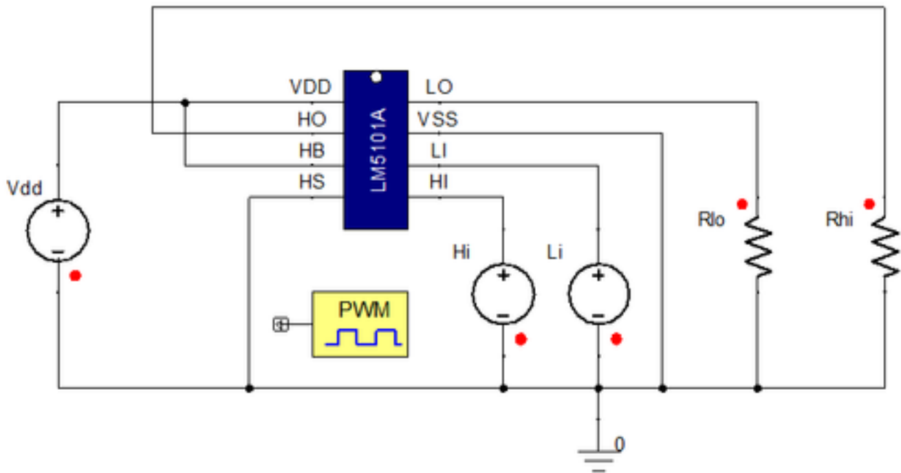
Figure 2. Example Circuit
