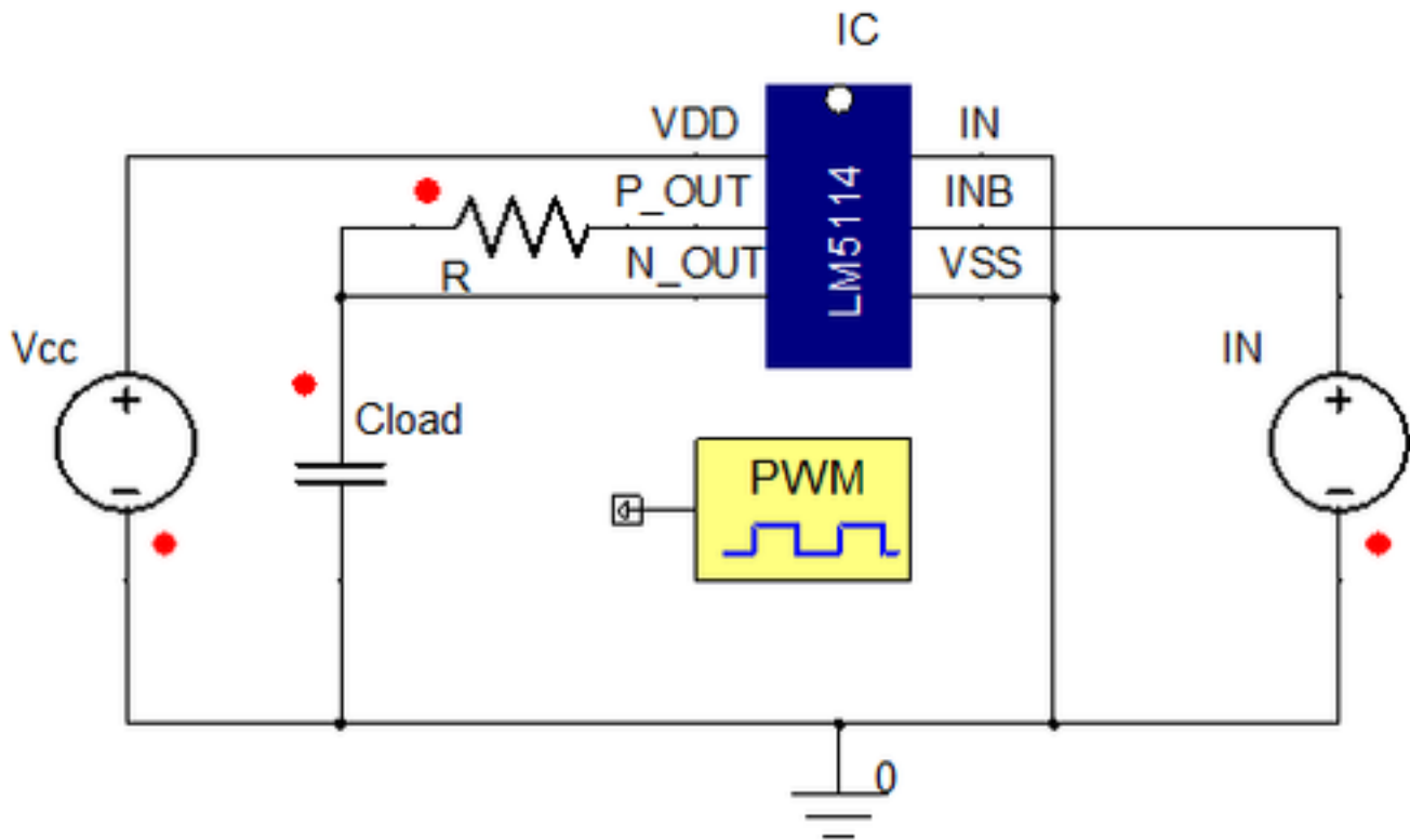
Figure 2. Example Circuit
