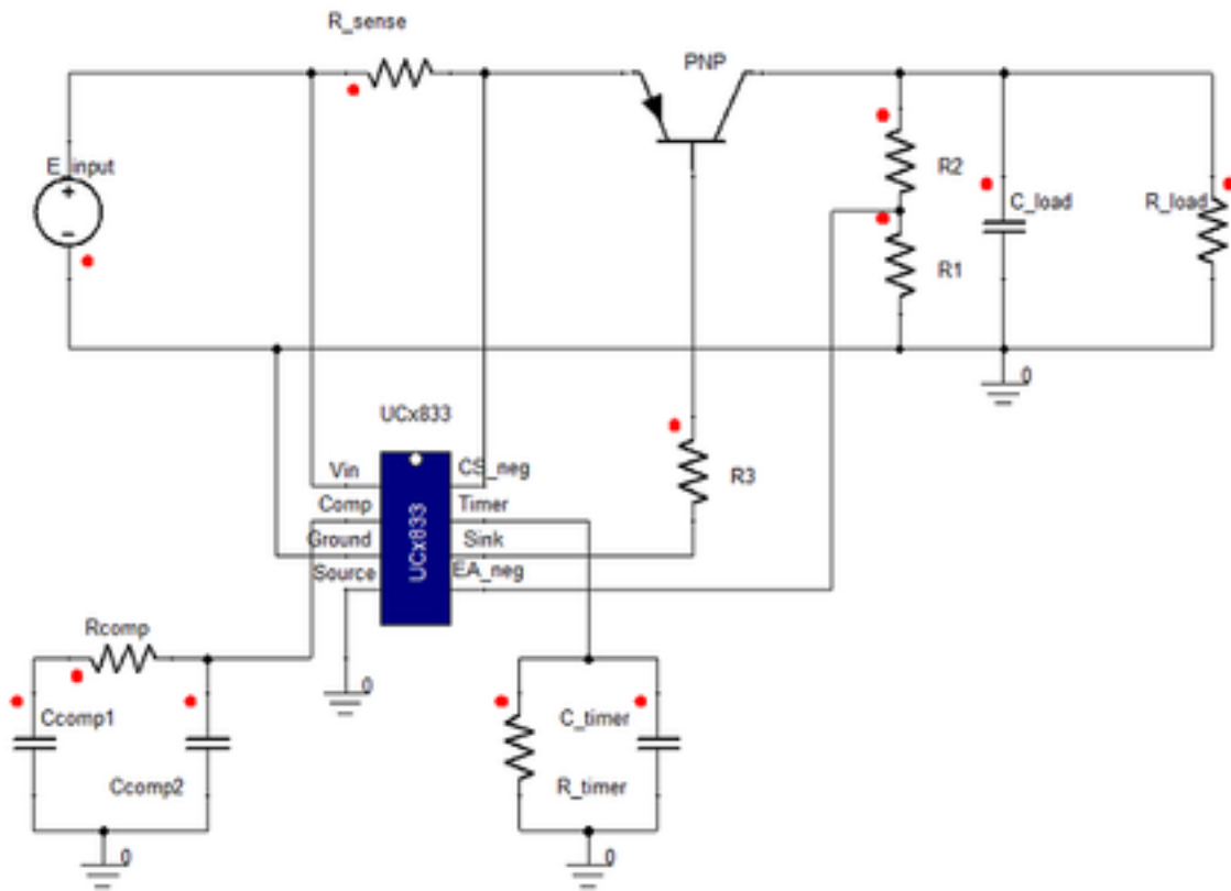
Figure 2. Example Circuit
