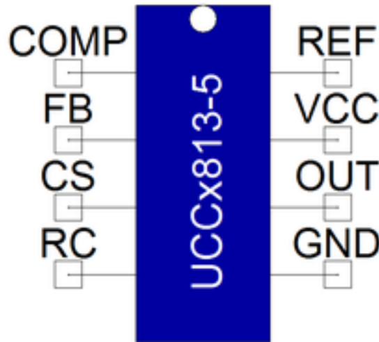
Figure 1. Component symbol
