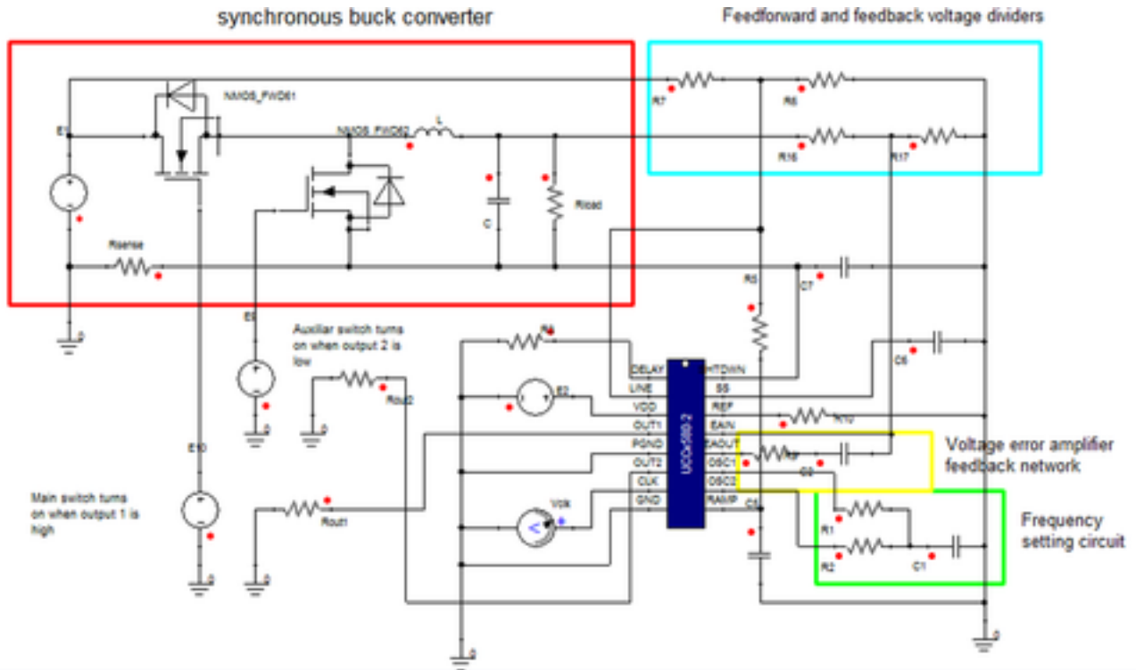
Figure 2. Example Circuit
